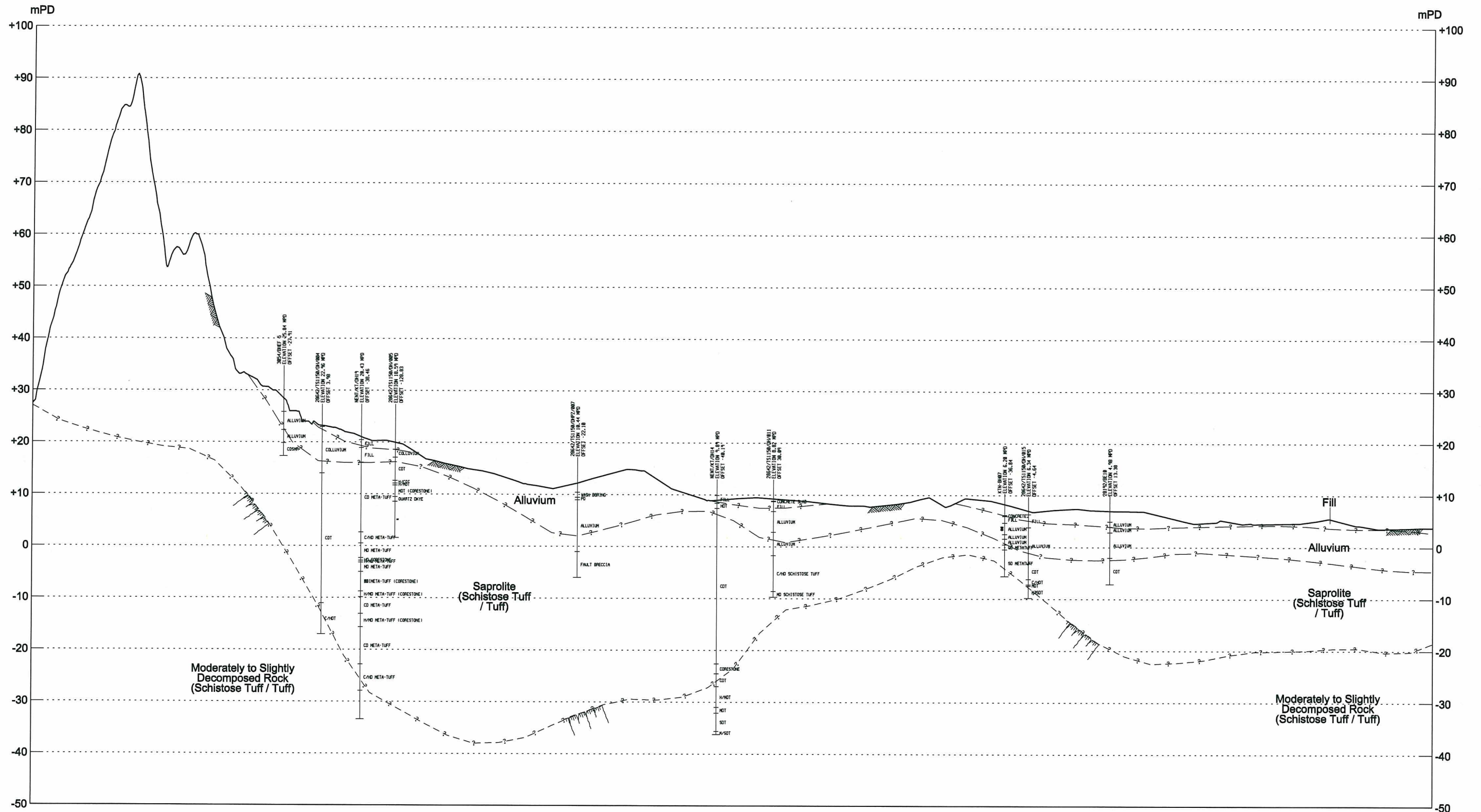
SECTION KTN06 SCALE H=1:7500 V=1:750 Fig. 3.3.1
