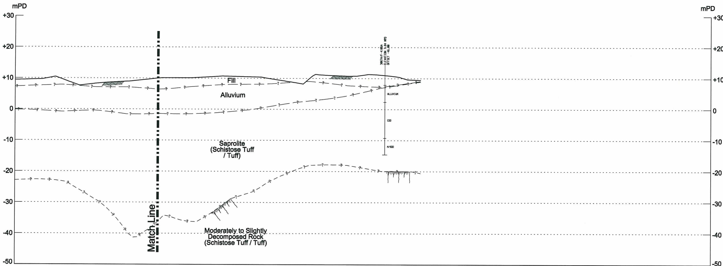
SECTION FLN02 SCALE H=1:7500 V=1:750 Fig. 3.3.2
