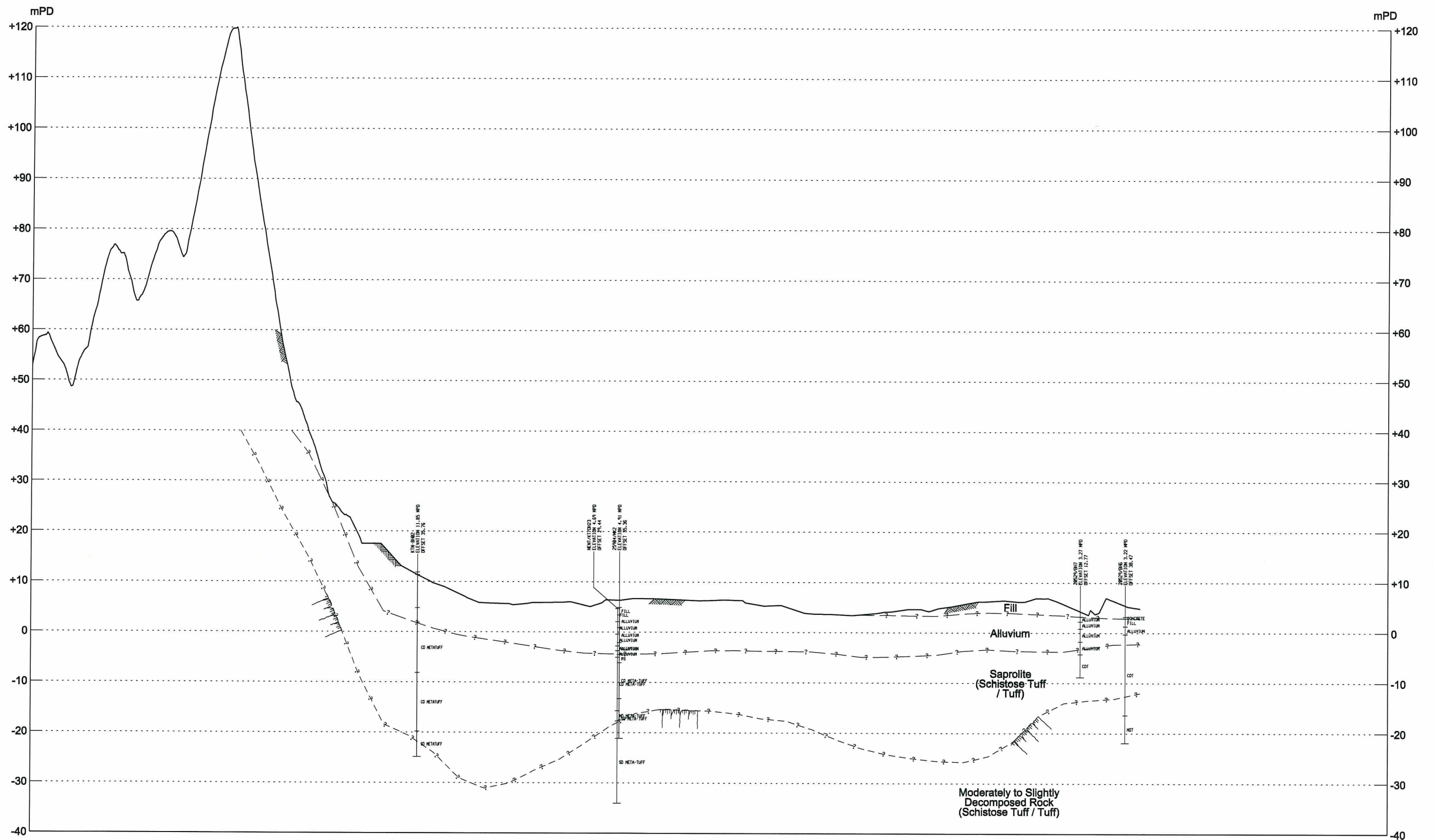
SECTION KTN09 SCALE H=1:7500 V=1:750 Fig. 3.3.1
