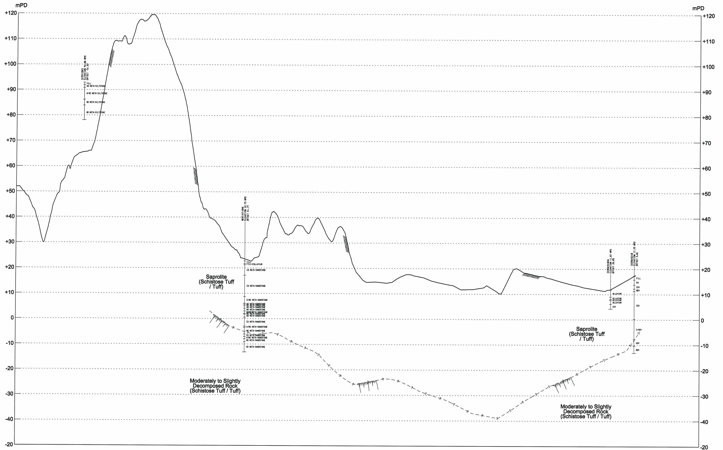
SECTION KTN10 SCALE H=1:7500 V=1:750 Fig. 3.3.1
