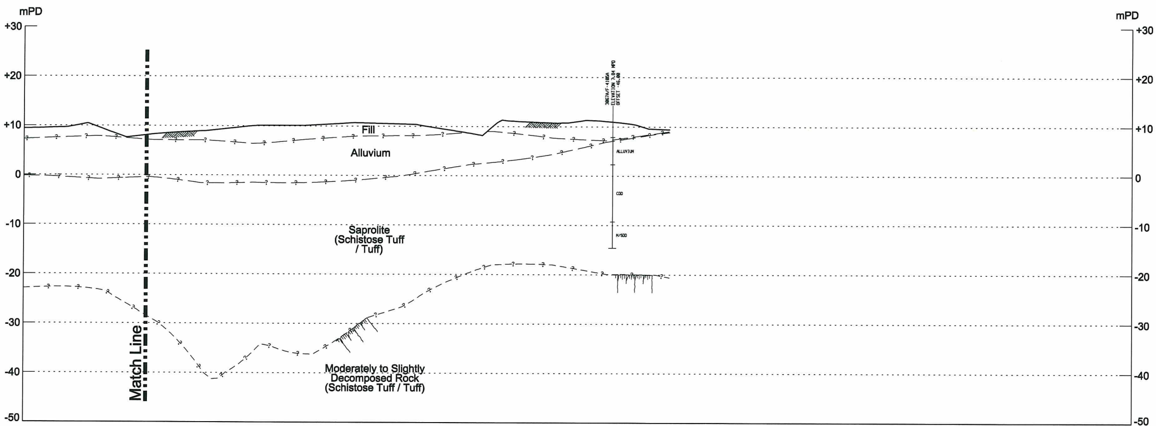
SECTION FLN06 SCALE H=1:7500 V=1:750 Fig. 3.3.2
