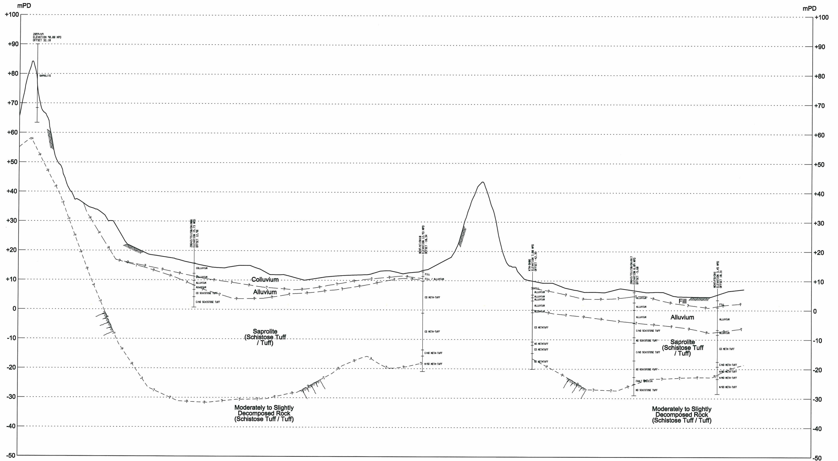
SECTION KTN02 SCALE H=1:7500 V=1:750 Fig. 3.3.1
