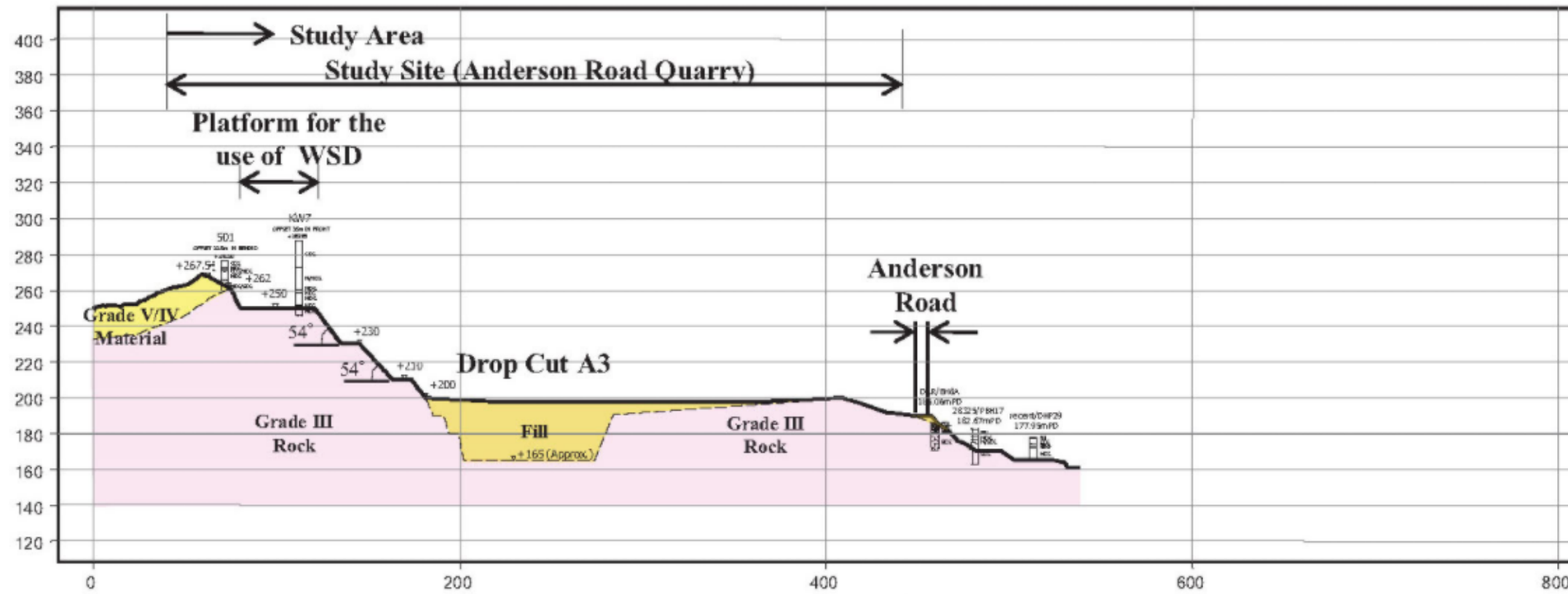
Section 1-1 (Planned Landform)
