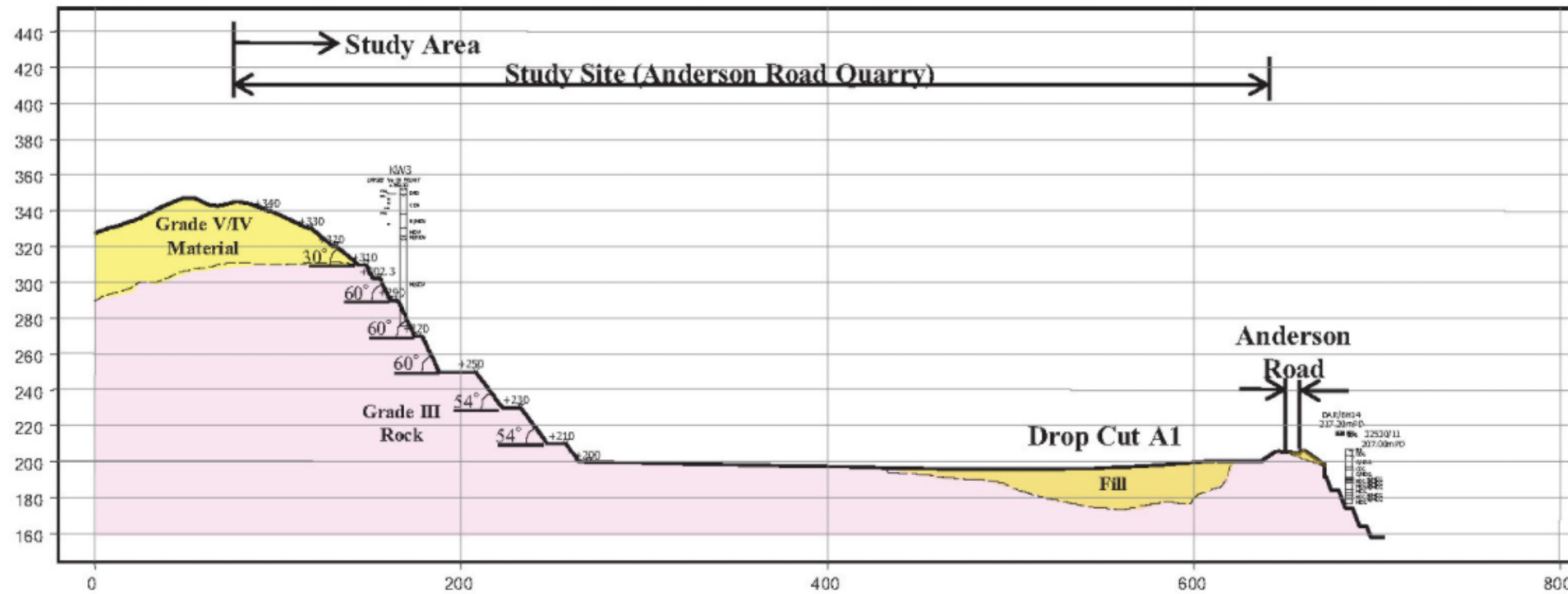
Section 2-2 (Planned Landform)
