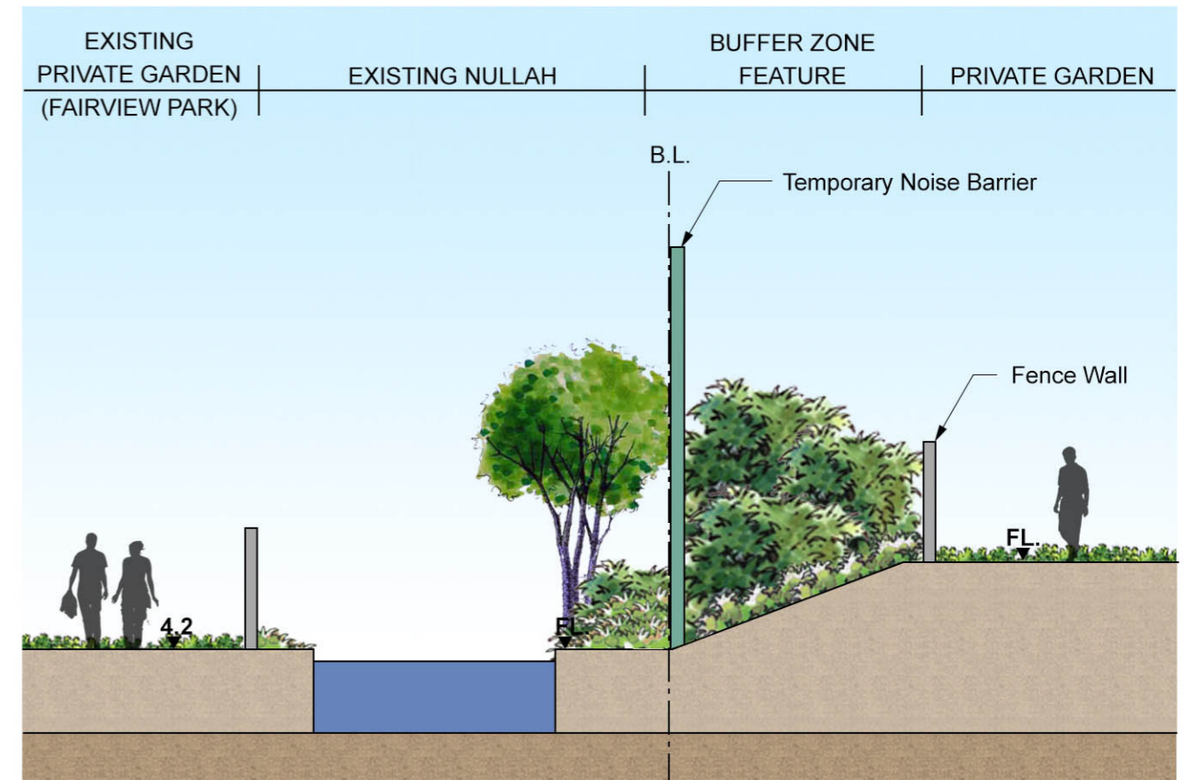
TYPICAL SECTION
