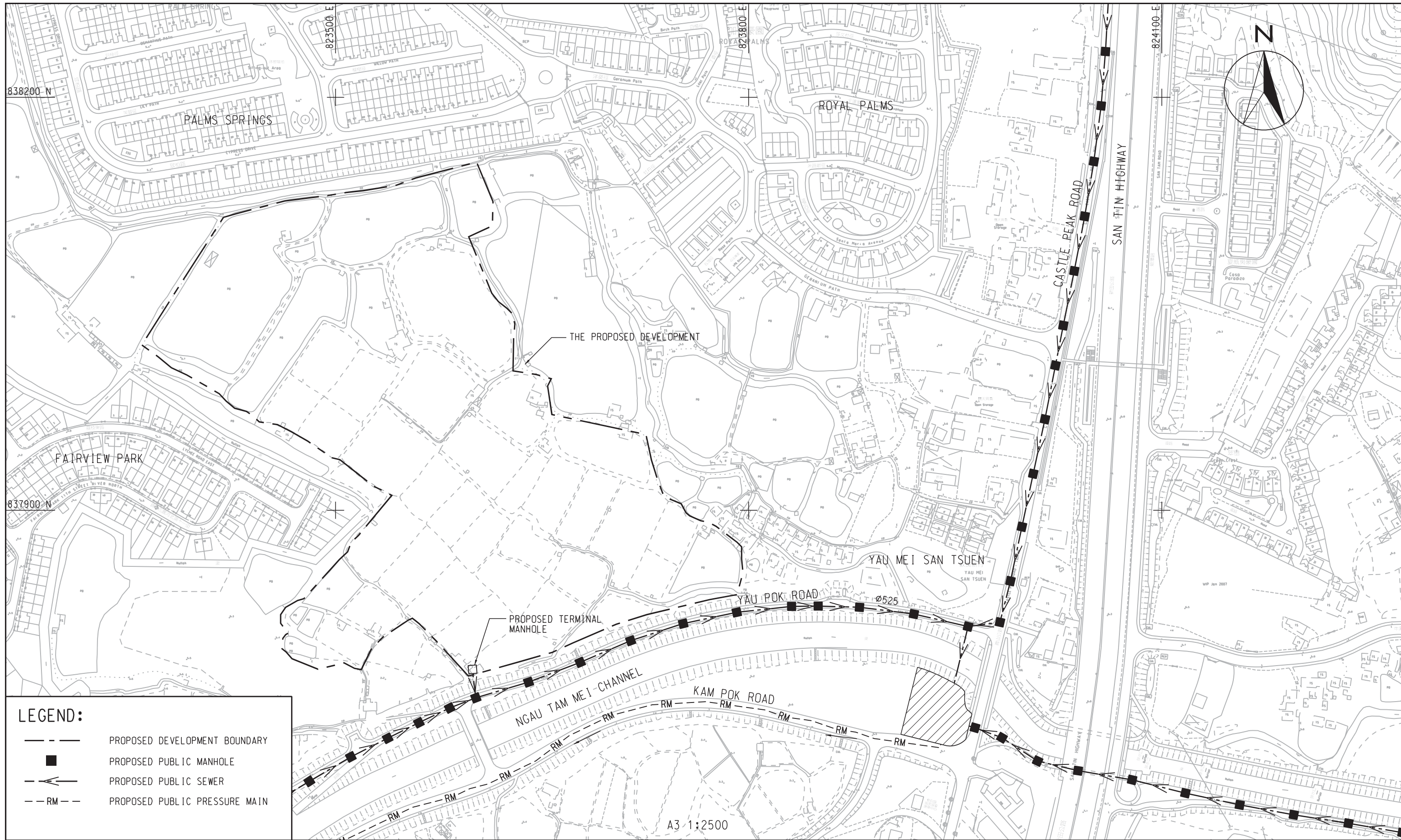
Figure: 6-2 Title: PROPOSED SEWER CONNECTION
