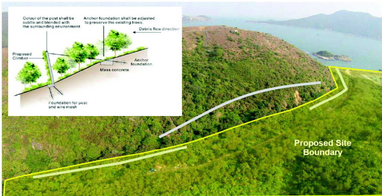
Approximate location of flexible barriers and schematic of arrangement
