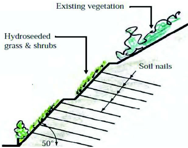
Schematic detail of slope nails and planting
