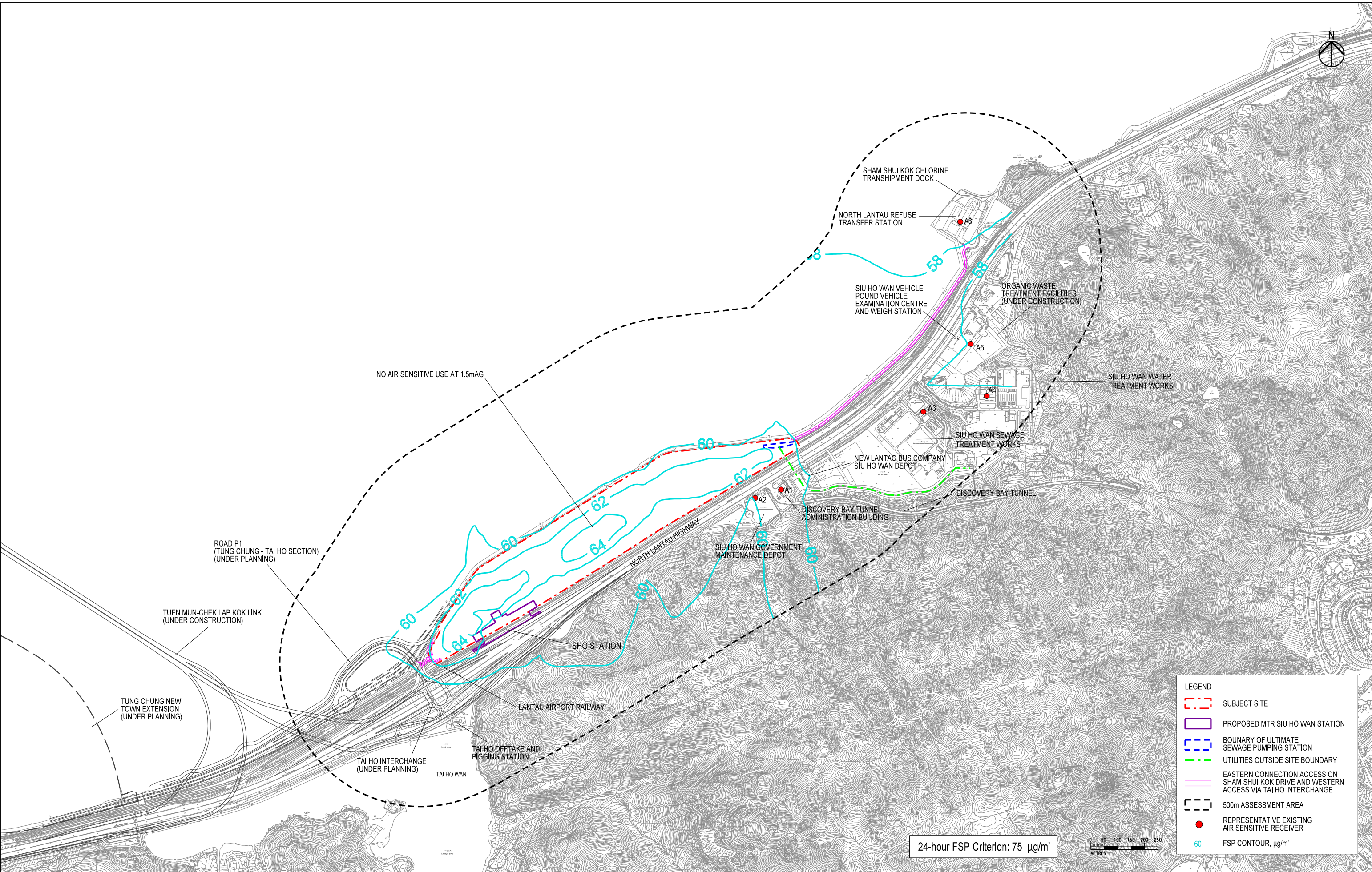
Proposed Comprehensive Residential and Commercial Development atop Siu Ho Wan Depot CONTOURS OF CUMULATIVE 10TH HIGHEST 24-HOUR FSP CONCENTRATION AT 1.5m ABOVE GROUND (OPERATIONAL PHASE)
