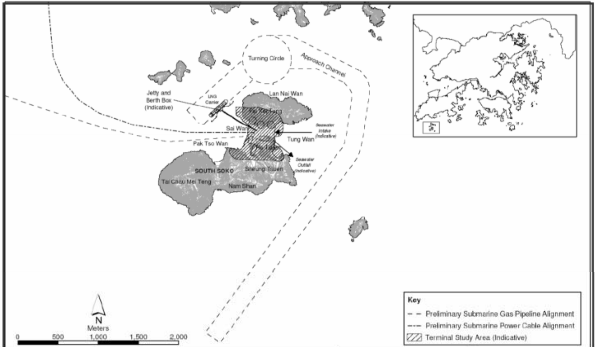
Appendix A1: Preliminary Conceptual Layout of South Soko LNG Terminal Project: Liquefied Natural Gas (LNG) Receiving Terminal and Associated Facilities ( Plan originated from Figure 2.4a of Project Profile )
