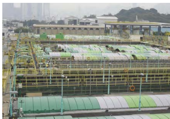
Covers at Stonecutters Island STW
