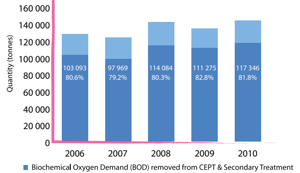
Removal of Organics in Sewage Treatment (2006-2010)
