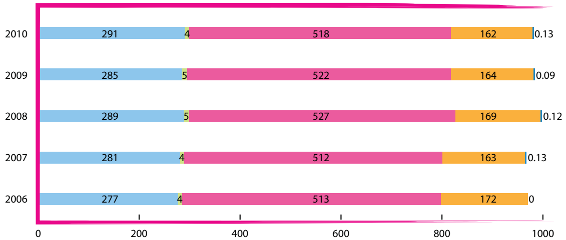
Distribution of Levels of Sewage Treatment (2006-2010) (in Mm 3 )
