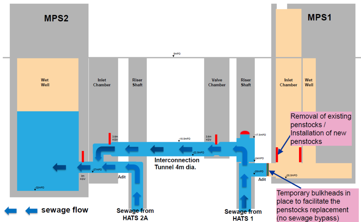
Figure E Removal / Installation of Penstocks in MPS1 (without Sewage Bypass)
