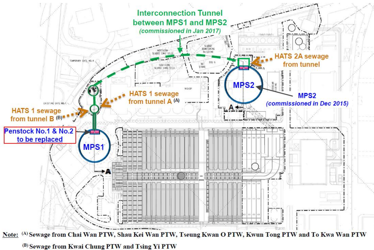
Figure B MPS1, MPS2 and the Interconnection Tunnel in SCISTW
