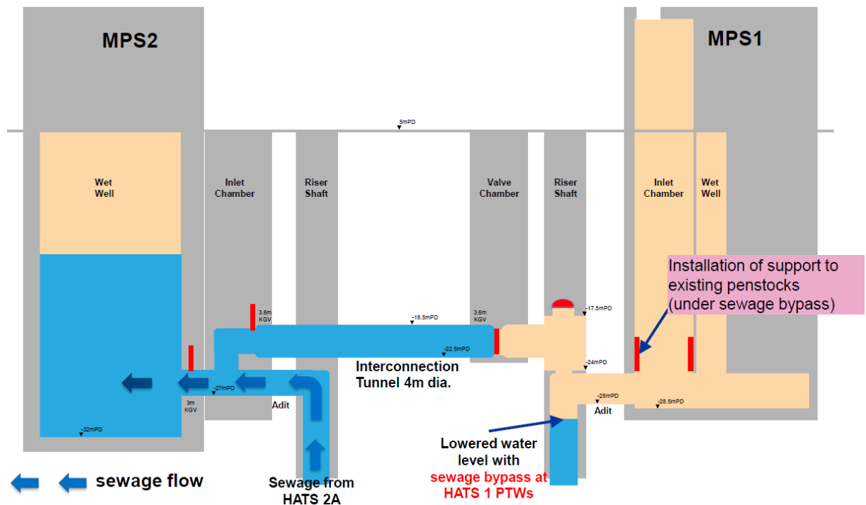
Figure C Installation of Temporary Support to Existing Penstocks (with Sewage Bypass)
