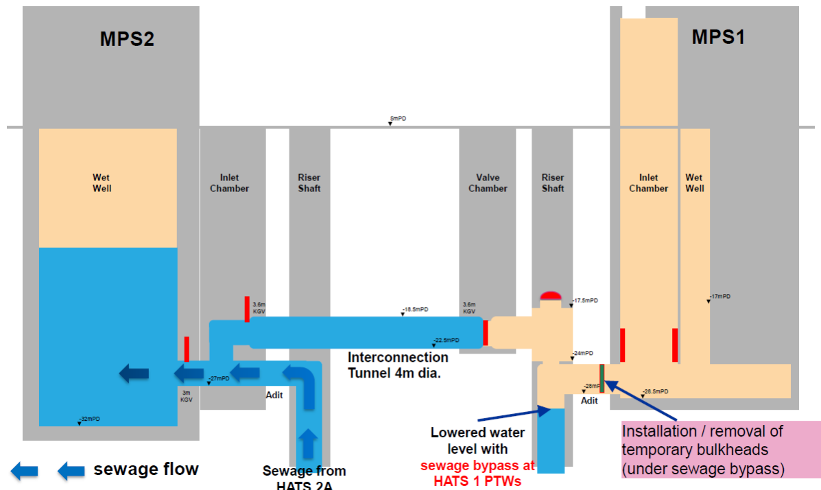
Figure D Installation / Removal of Temporary Bulkheads (with Sewage Bypass)
