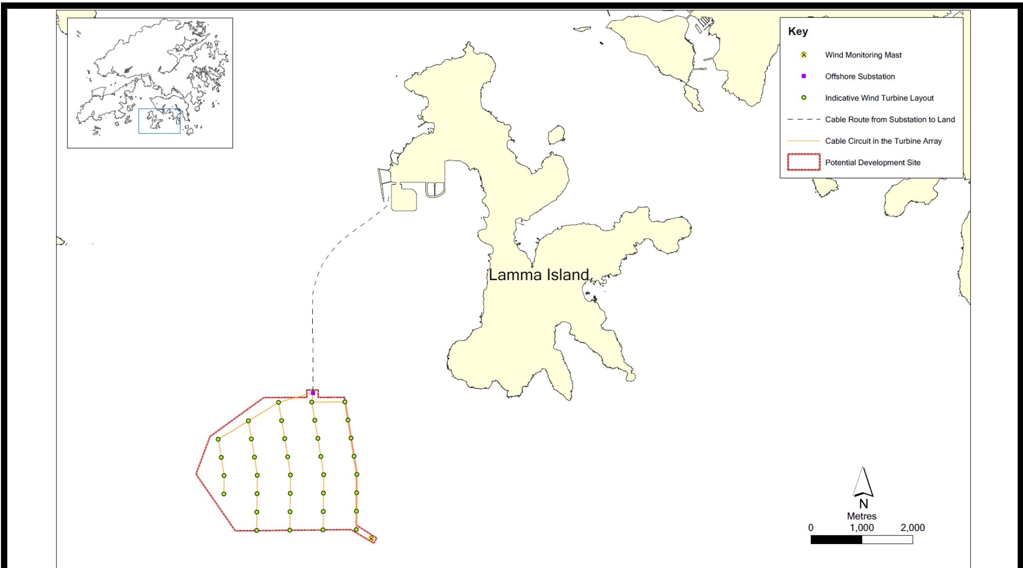
Project Title: Development of a 100MW Offshore Wind Farm in Hong Kong Location of the Project (Reproduced from Figure 5.1 of the EIA Report)
