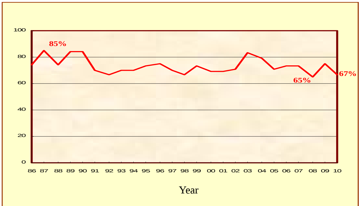
Figure 3 - Overall compliance with the Marine Water Quality Objectives in the Southern WCZ, 1986-2010
