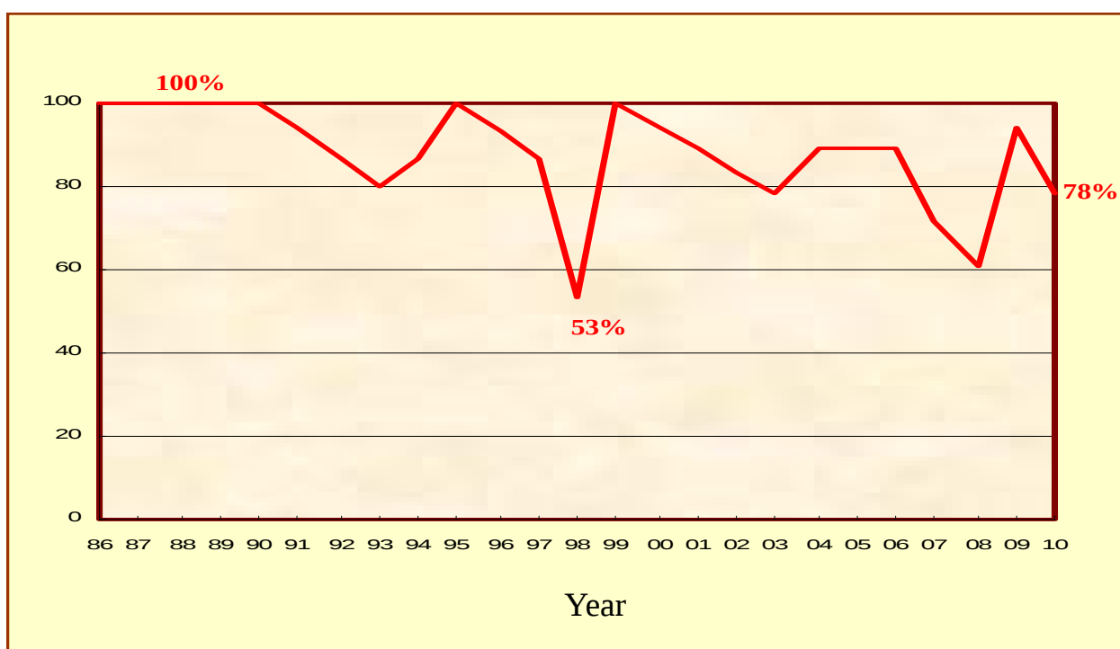
Figure 2 - Overall compliance with the Marine Water Quality Objectives in the North Western WCZ, 1986-2010
