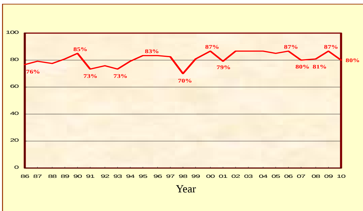
Figure 1 - Overall compliance with the Marine Water Quality Objectives in Hong Kong, 1986-2010
