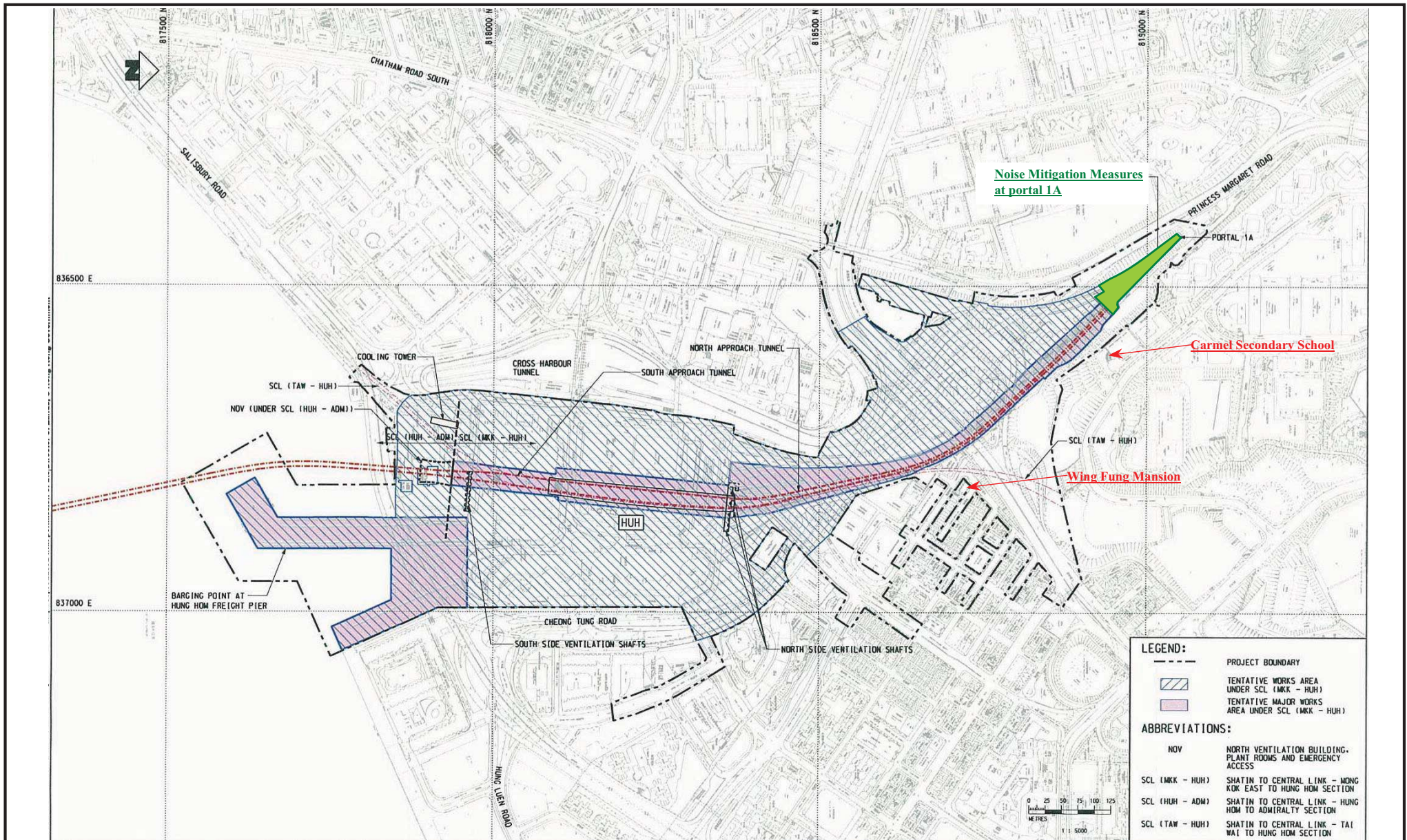
Figure 1: Overall View of Alignment & Works Sites
