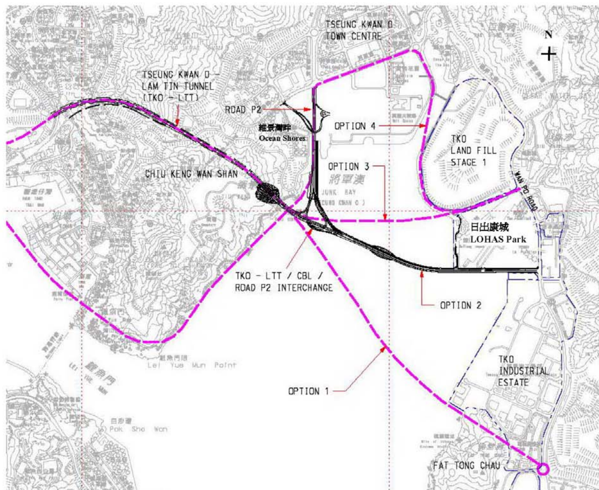
Figure 2: Cross Bay Link Alignment Options Project Title: Cross Bay Link, Tseung Kwan O
