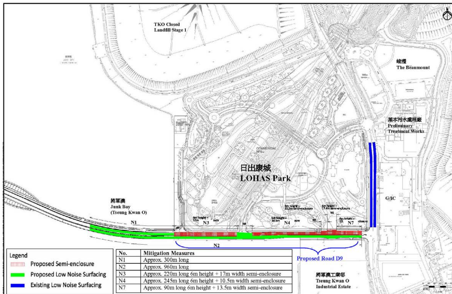
Figure 3: Noise Mitigation Package Project Title: Cross Bay Link, Tseung Kwan O
