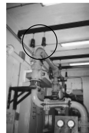
Installation of Spring Hangers (Noise Reduction: 8dB(A))
