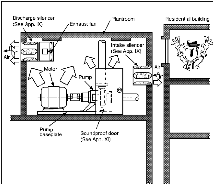
Figure 9 : Plantroom for Pumpsets
