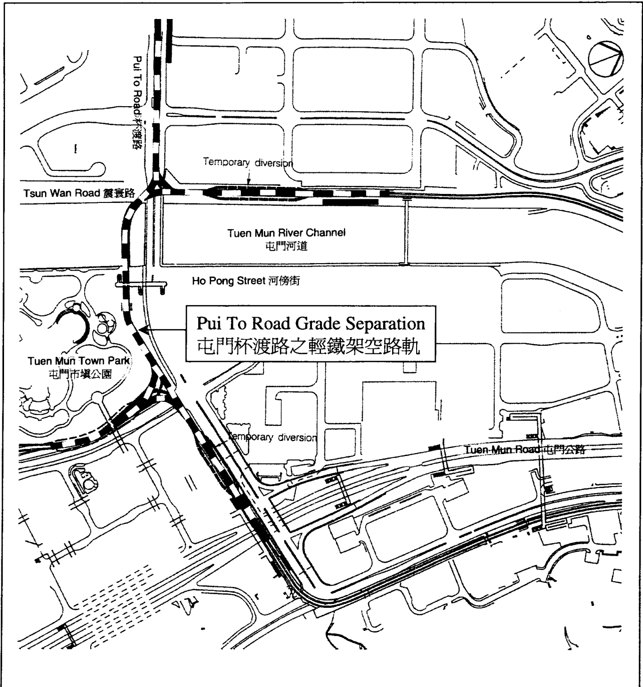
Figure 2 Location Plan 地點圖 附圖二 Pui To Road Grade Separation 屯門杯渡路之輕鐵架空路軌
