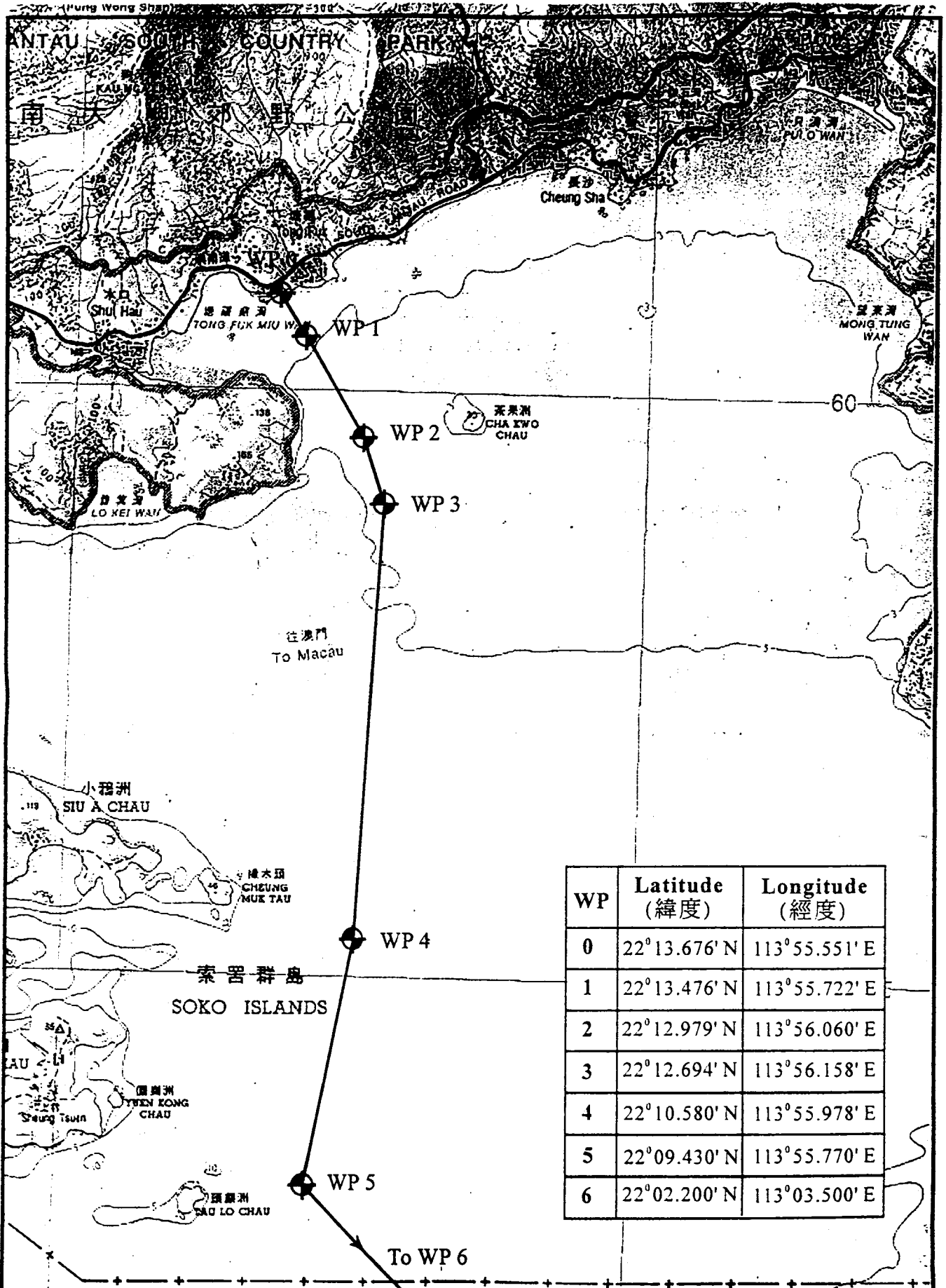
Figure 1 NAC Telecommunication Cable Alignment
