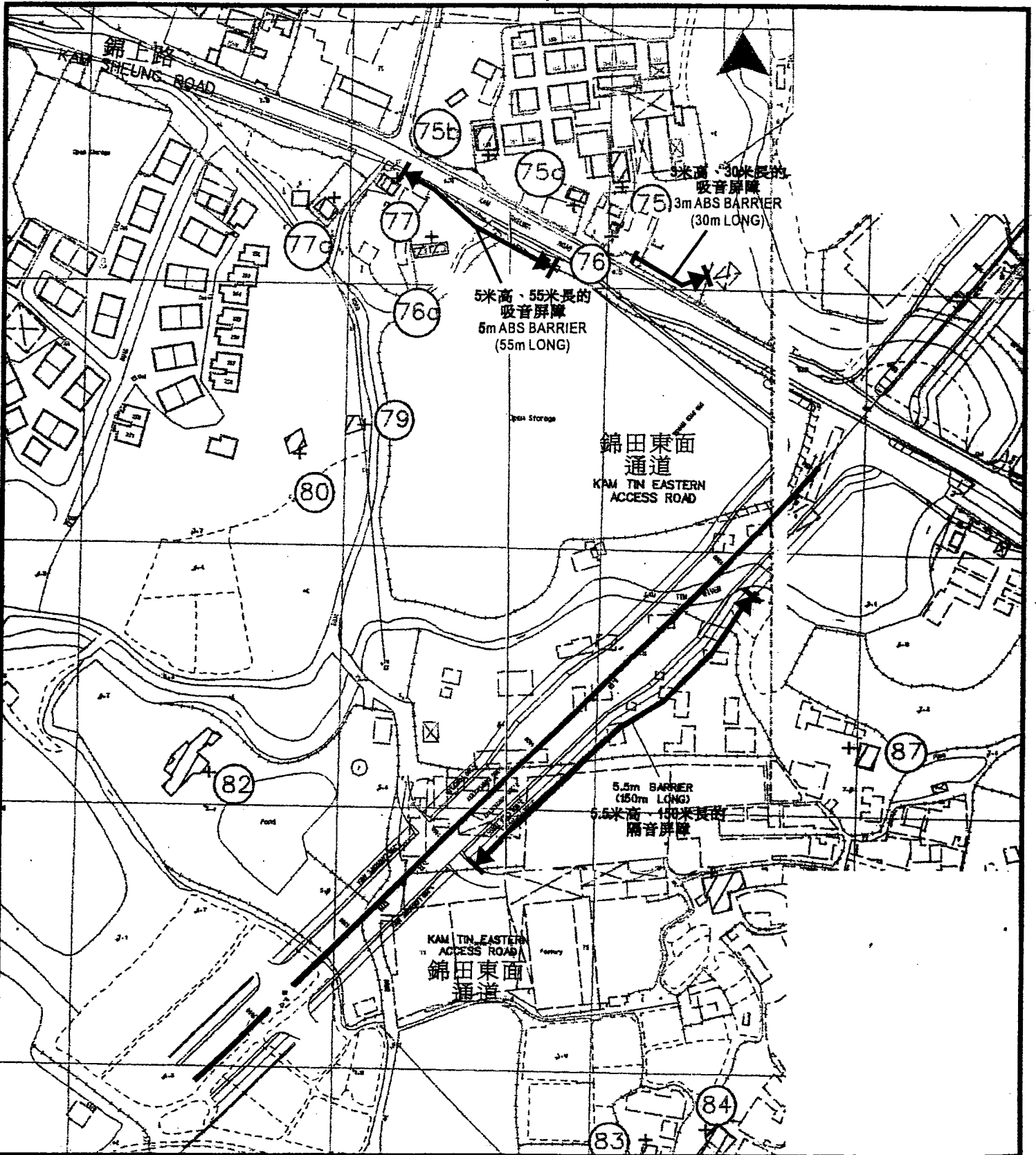
Figure 3 - Direct Road Traffic Noise Mitigation Measures For Kam Tin Eastern Access Road (South & West Section)
