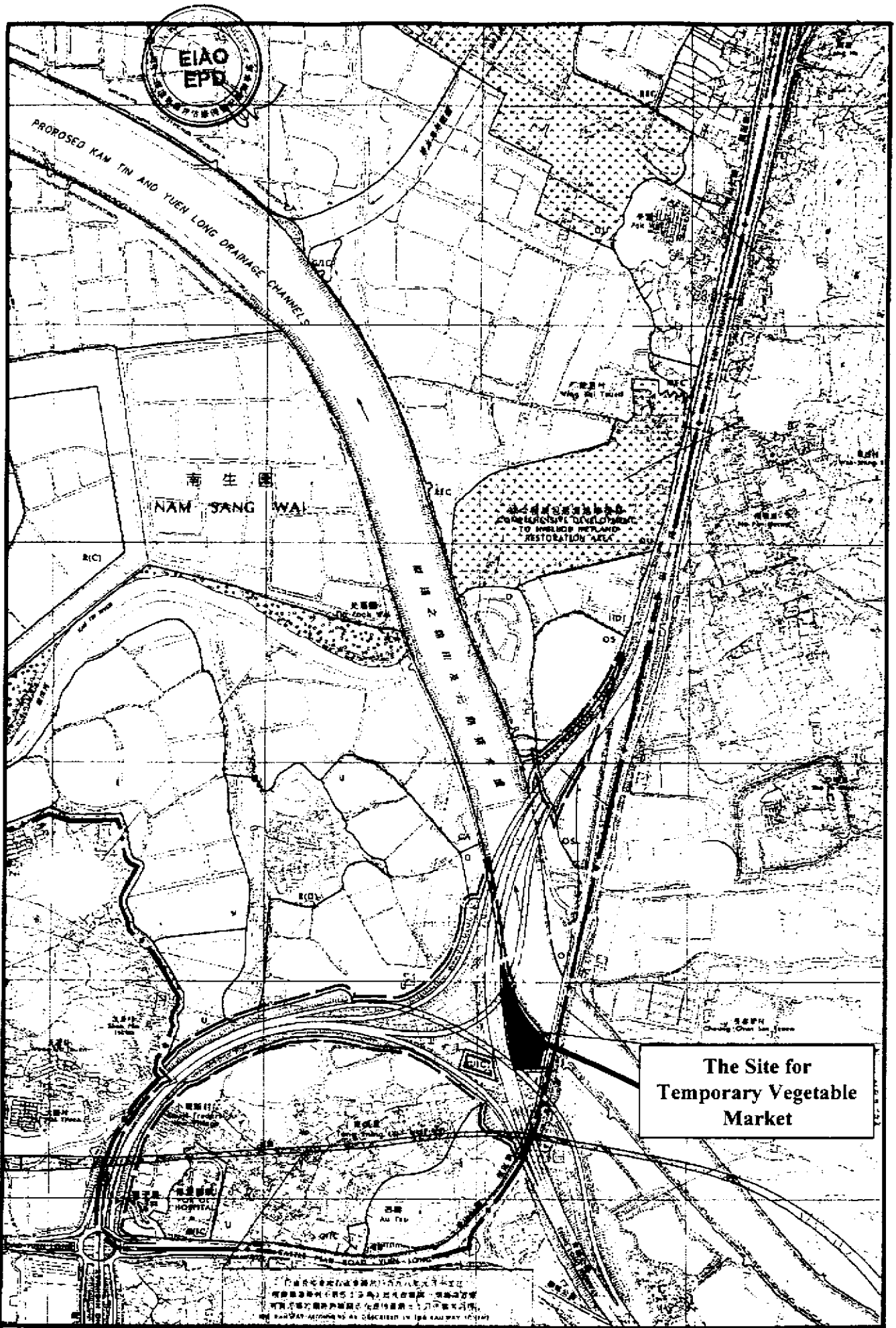
Figure 1 Location Plan for the Temporary Vegetable Market at Nam Sang Wai Road, Au Tau, Yuen Long
