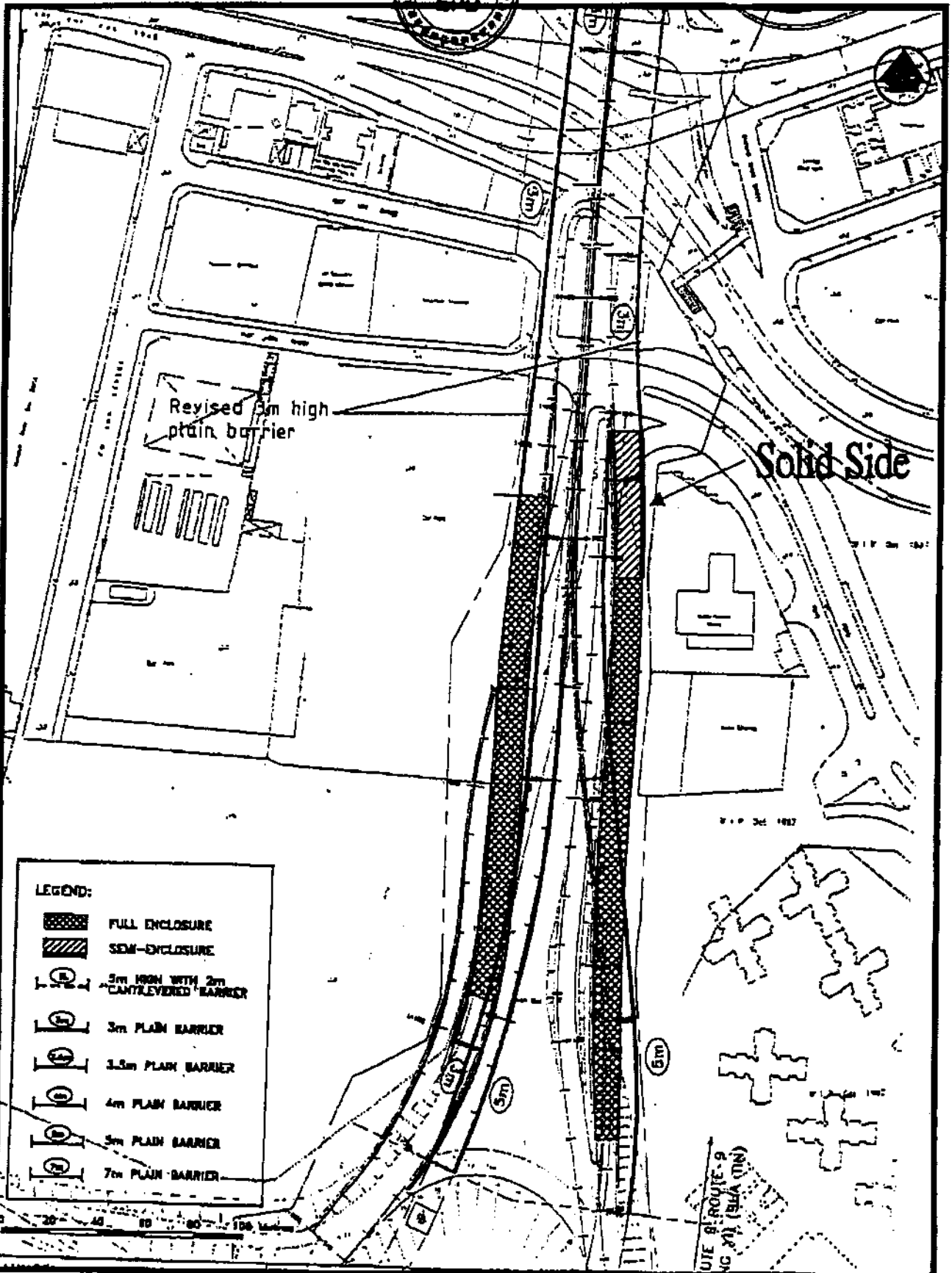
Figure 2 Noise Barriers and Enclosures (Extracted from the Application AEP-103/2001)
