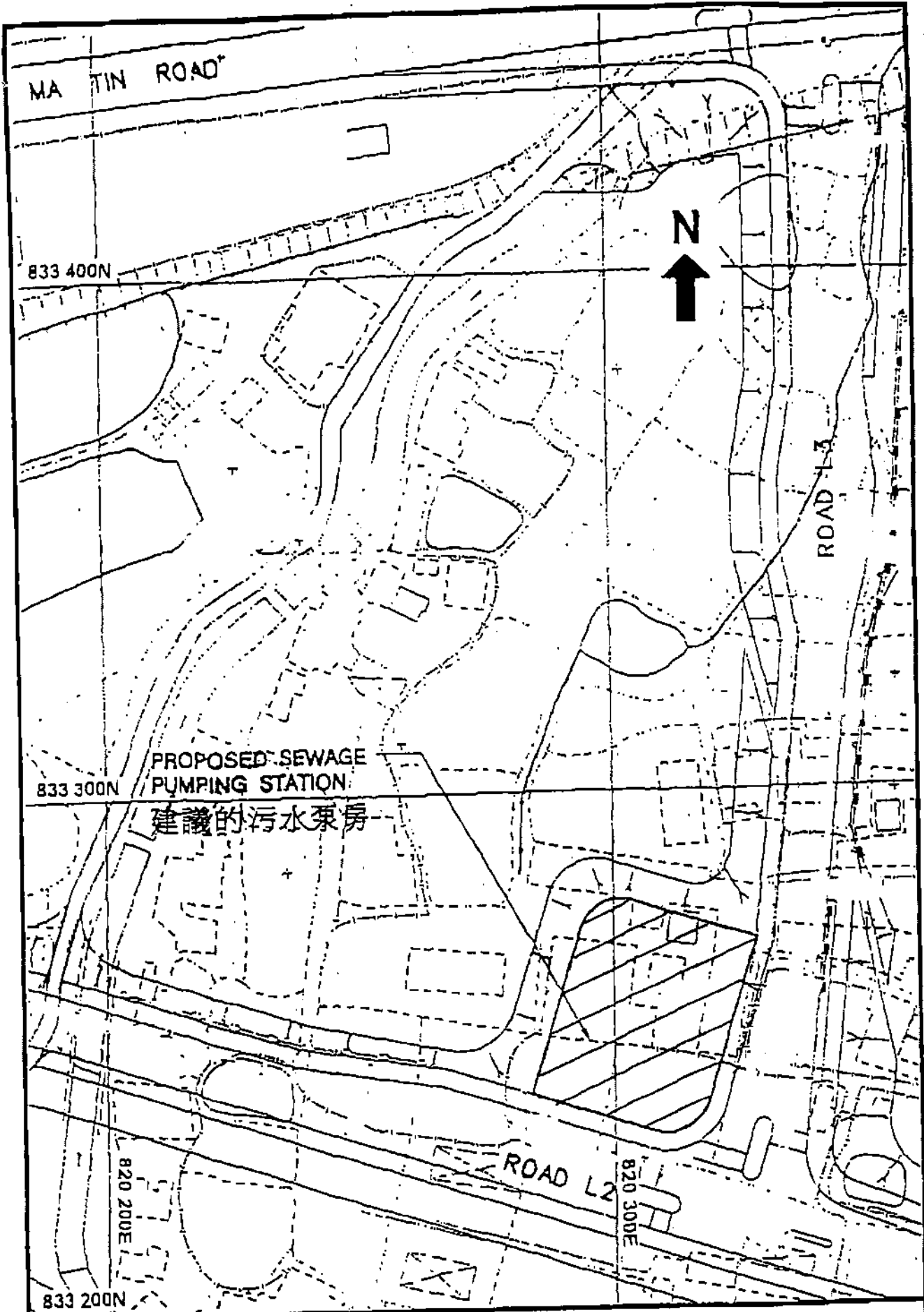
Figure 1 - Location Plan of Yuen Long Area 13 Sewage Pumping Station
