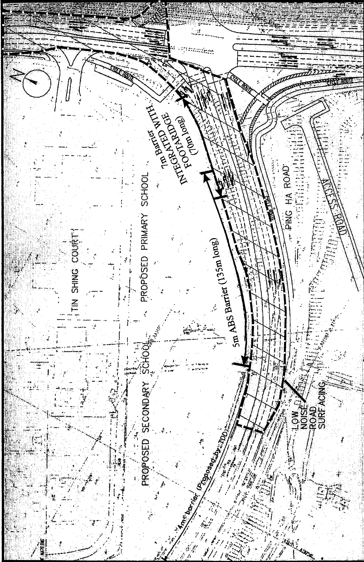
FIGURE 5 - Proposed Direct Road Traffic Noise Mitigation Measures on Ping Ha Road, Tin Shui Wai
