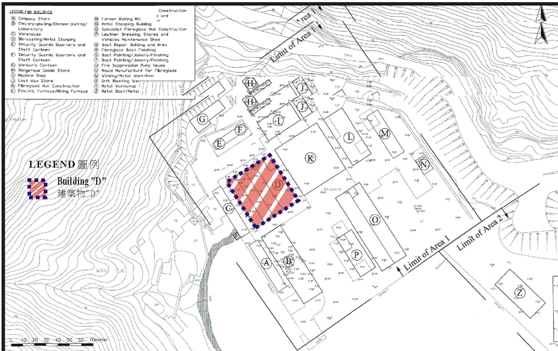
Figure 3 Location of Building D in Cheoy Lee Shipyard Site
