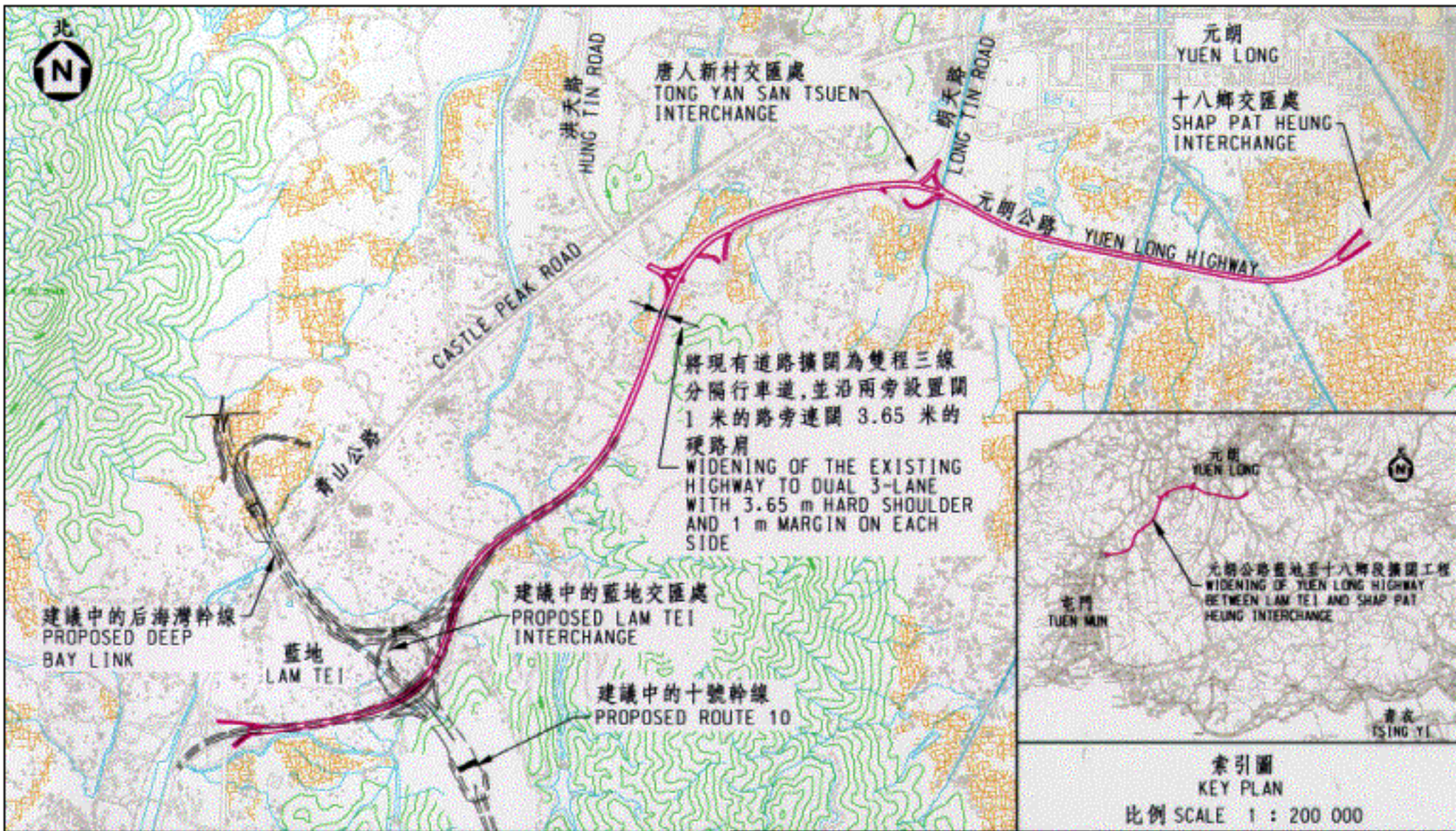
Widening of Yuen Long Highway between Lam Tei and Shap Pat Heung Interchange
