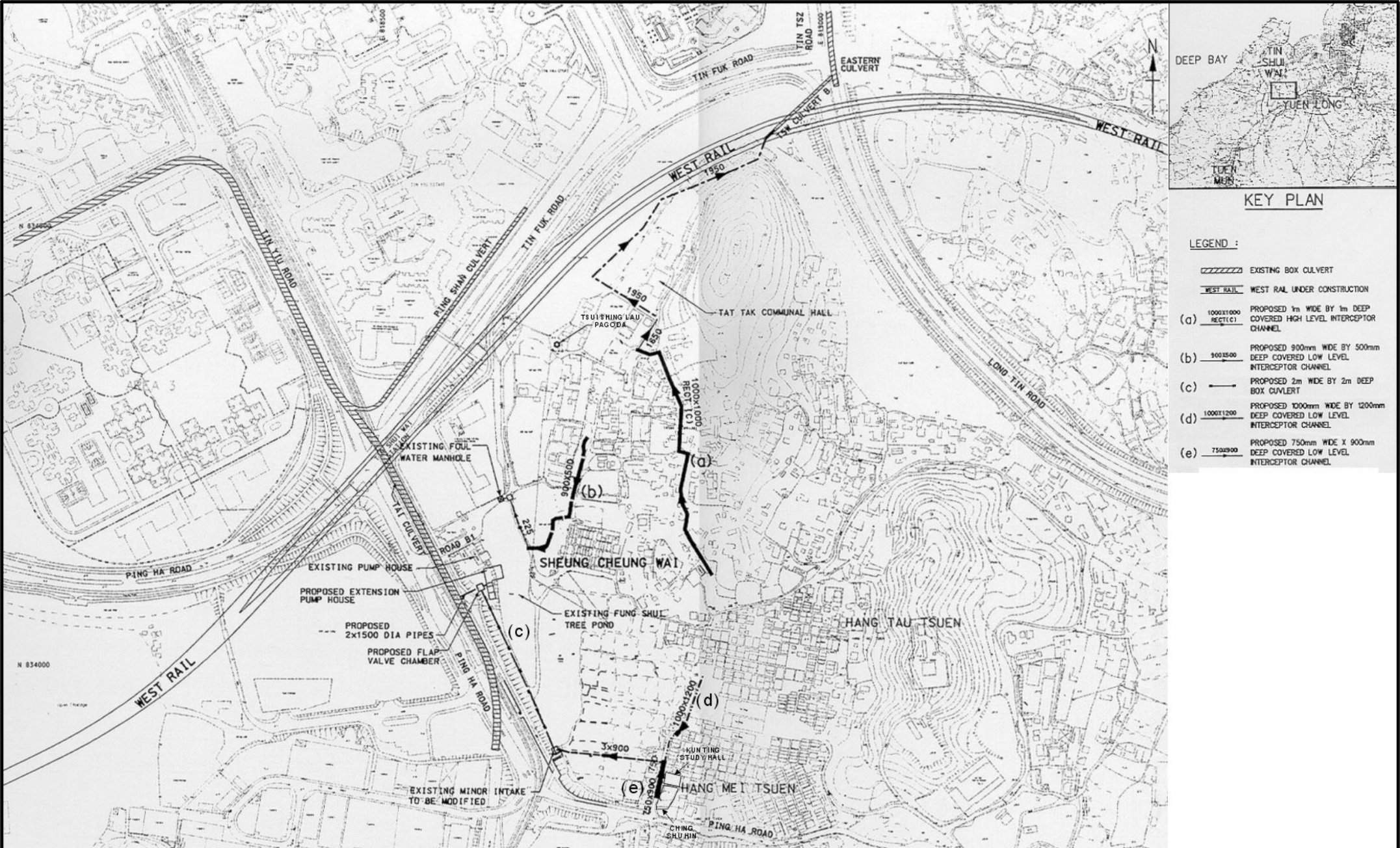
Figure 1 - Village Flood Protection Works For Sheung Cheung Wai
