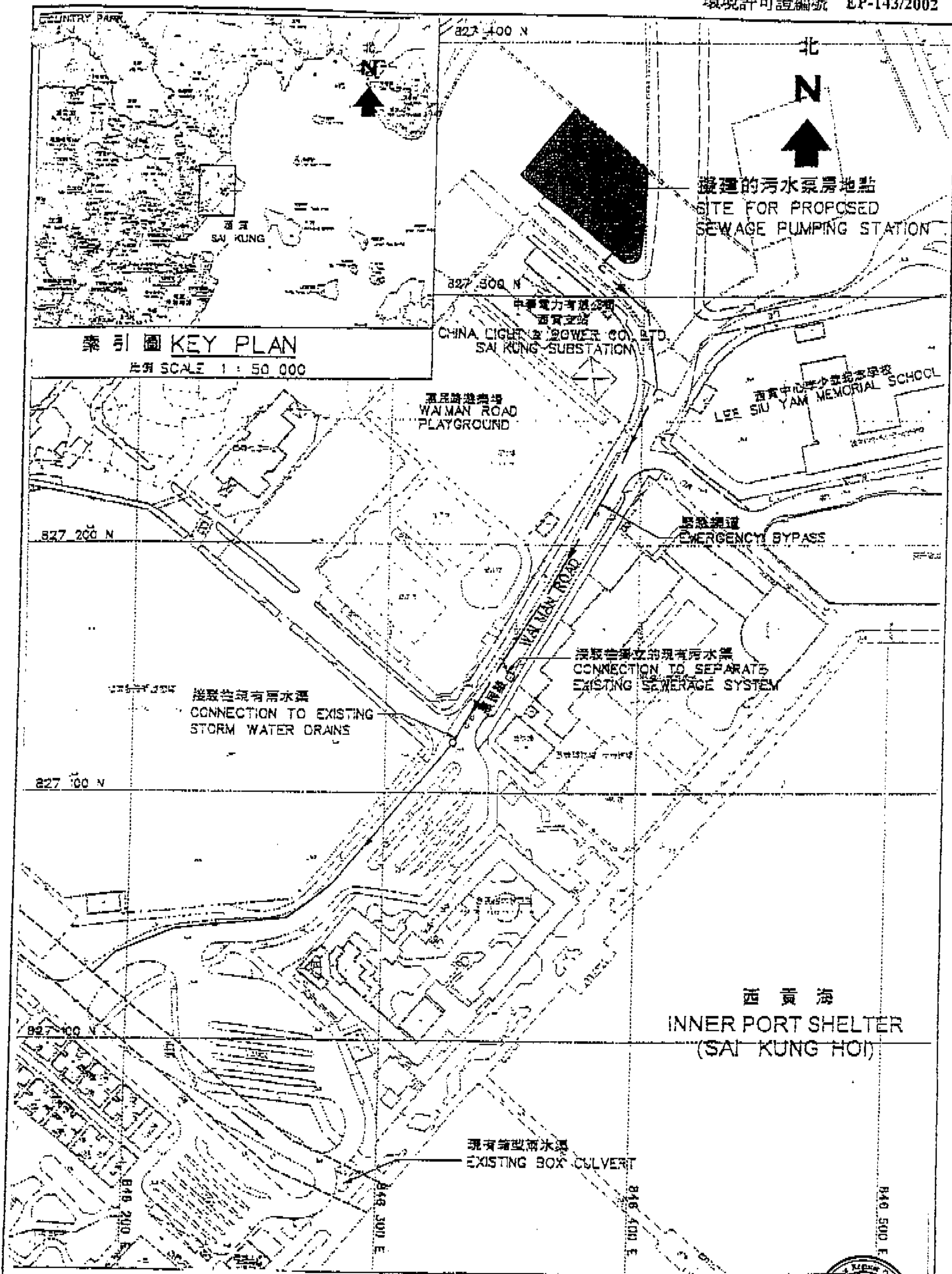
Drawing No. 1 : Sai Kung Area 4 Sewage Pumping Station - Location of Proposed Sewage Pumping Station 圖則編號 1 : 西貢第 4 區污水泵房擬建的污水泵房位置圖
