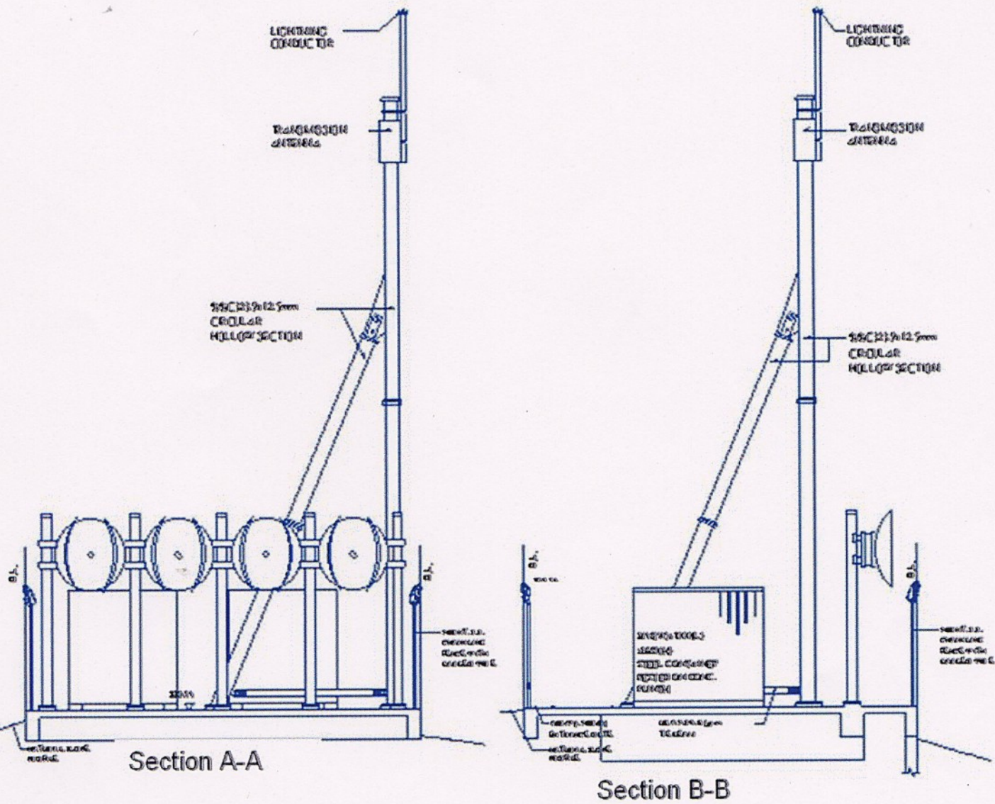
Figure 4 - Section View of the Project
