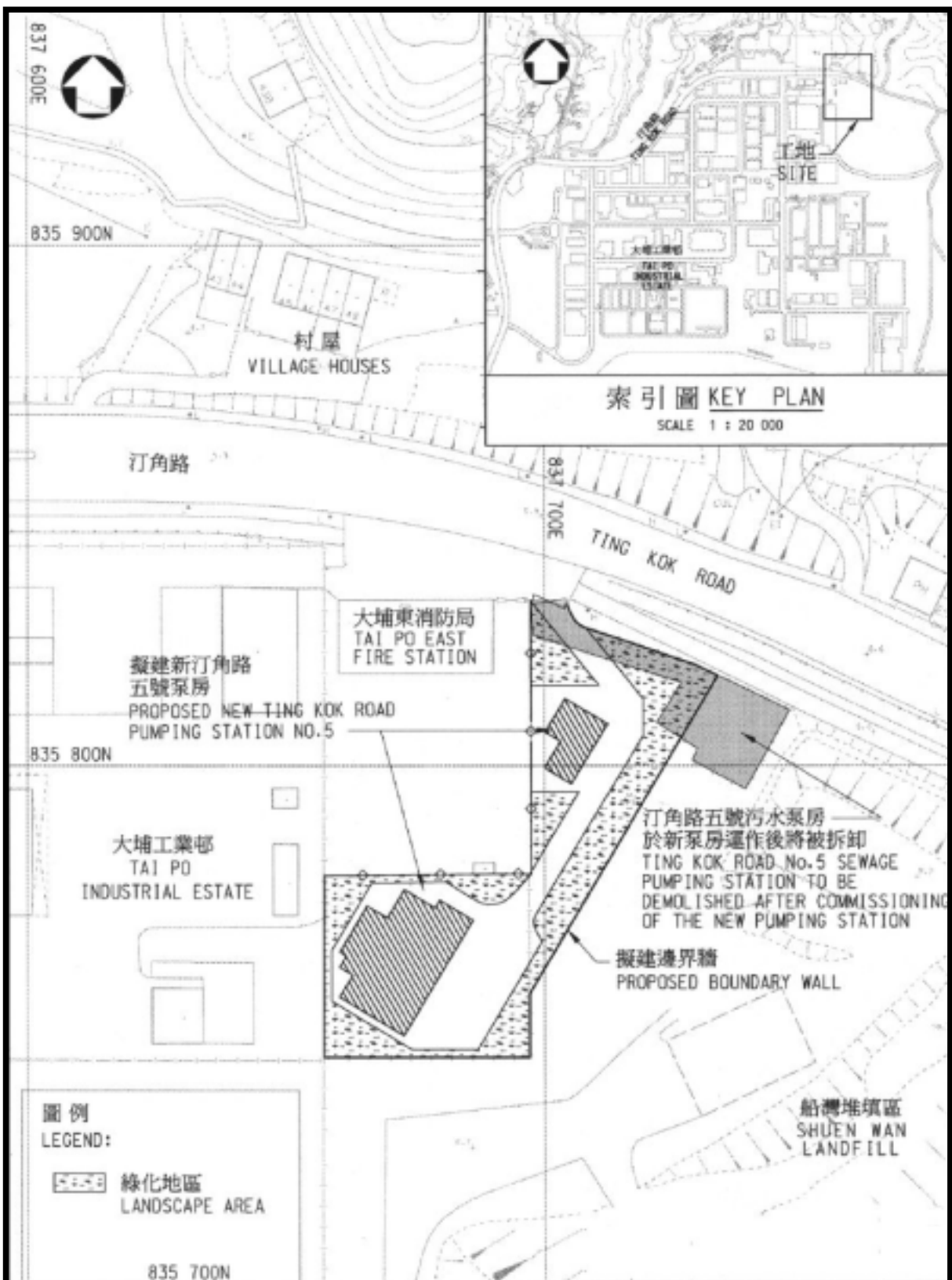
Figure 1 Upgrading of Ting Kok Road Pumping Station No.5
