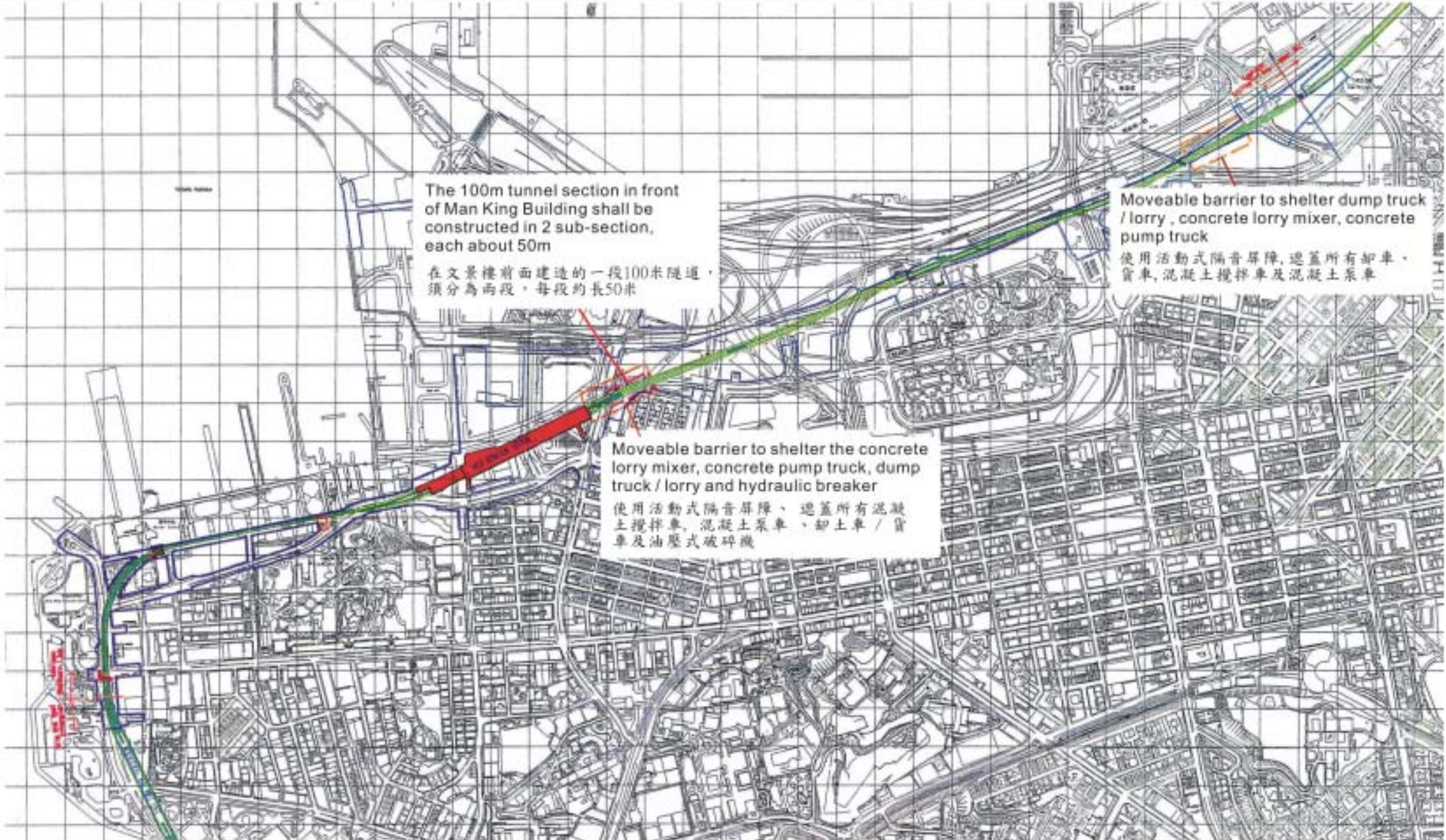
Figure 3 : Specific Mitigation Measures for Particular Powered Mechanical Equipments at Worksites in front of Man King Building and Olympian City Phase III
