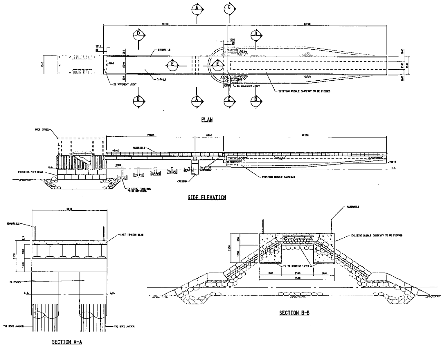
Figure 2: Improvement Works to Tung Ping Chau Public Pier – General Arrangement
