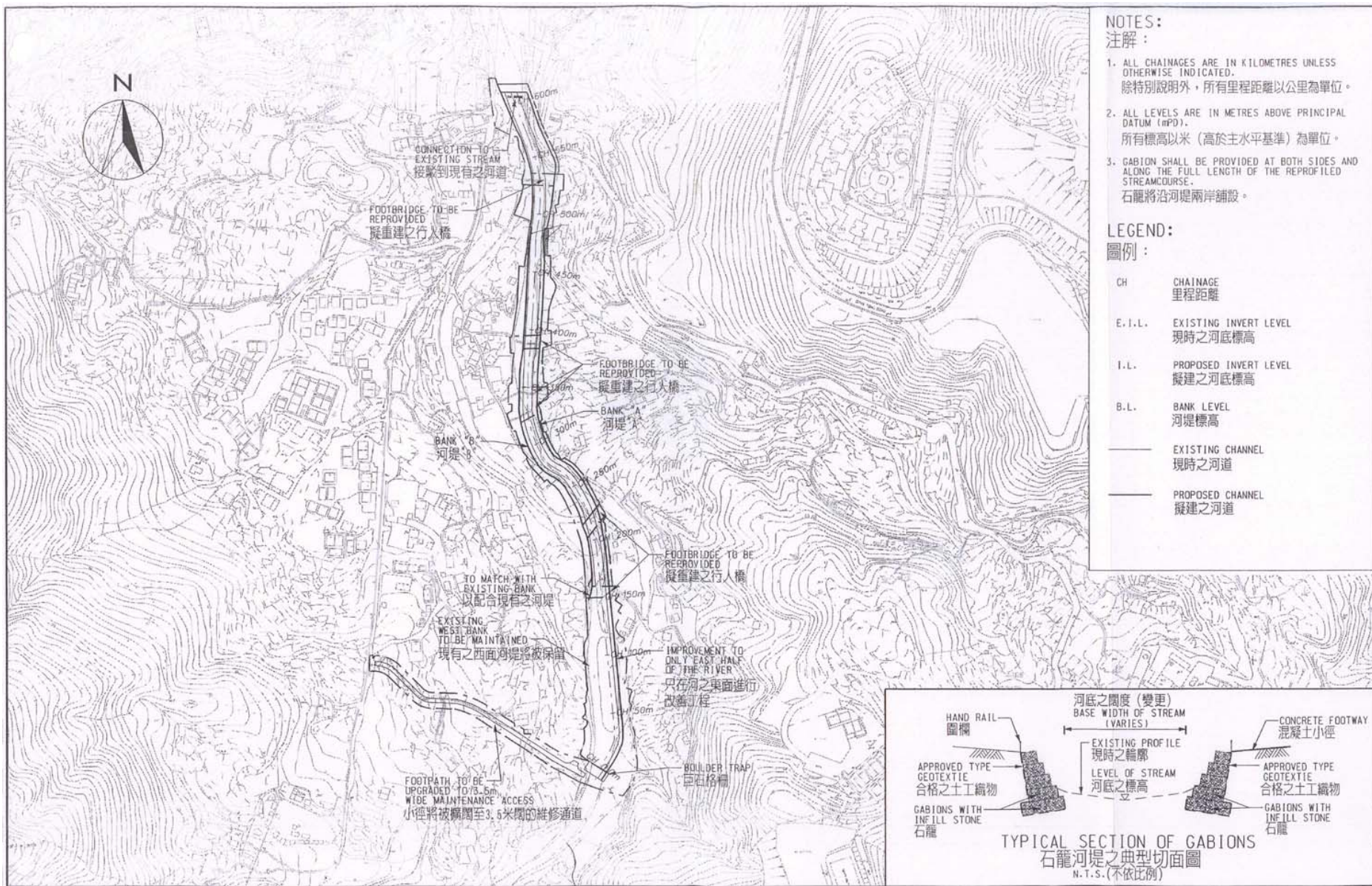
Figure 2: Drainage Improvement Works in Upper Tai Po River – General Layout Plan
