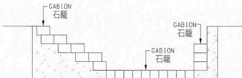
石籠襯砌梯形排水道 TRAPEZOIDAL CHANNEL WITH GABION BASE AND WALL
