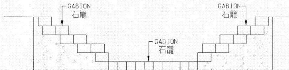
石籠襯砌梯形排水道 TRAPEZOIDAL CHANNEL WITH GABION BASE AND WALL
