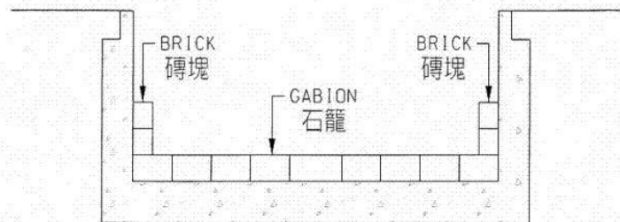
石籠磚塊襯砌方形排水道 RECTANGULAR CHANNEL WITH GABION BASE AND BRICK WALL
