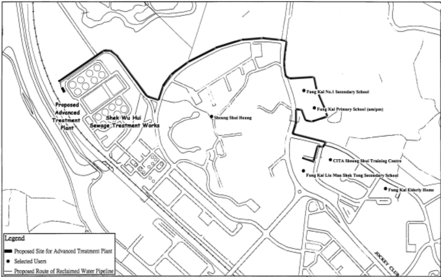
Figure 1 - Demonstration Scheme on Reclaimed Water Uses in the North District – Project Layout
