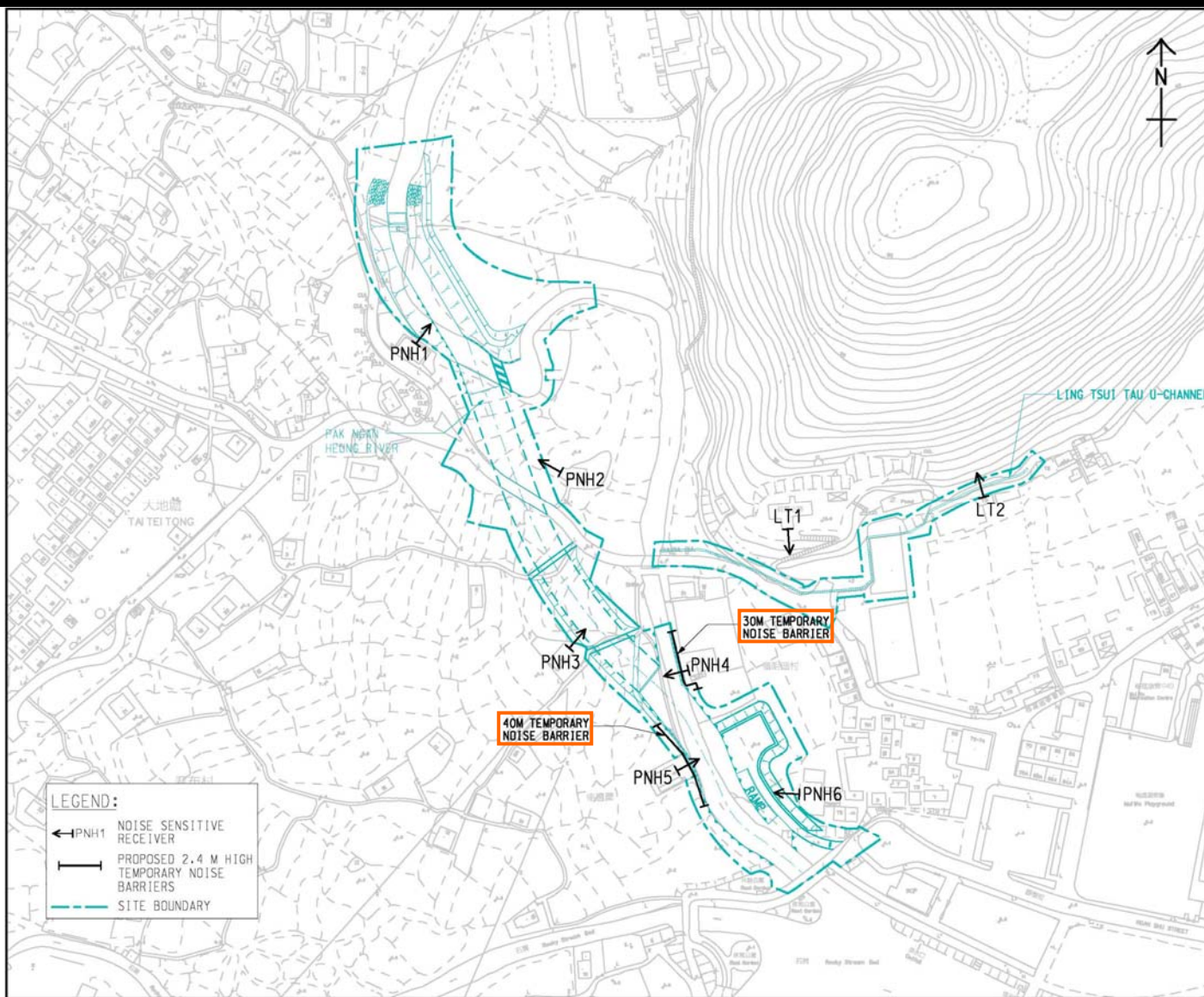
Figure 3: Locations of Temporary Noise Barriers (Ref. Drg. No. 4.2, sheet 1 of 2, of the EIA Report)
