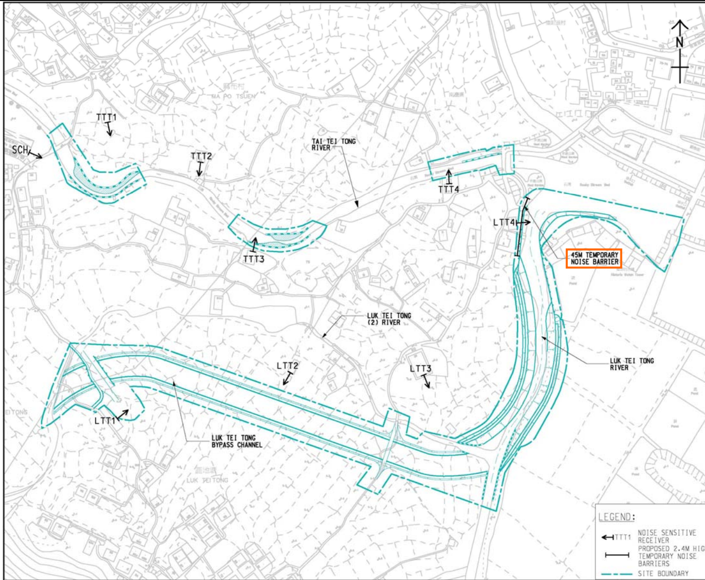
Figure 4: Locations of Temporary Noise Barriers (Ref. Drg. No. 4.2, sheet 2 of 2, of the EIA Report)
