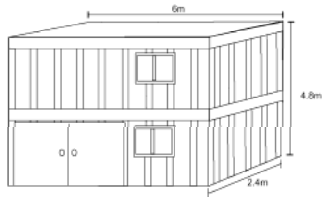
Typical Structure for Kart Maintenance Purpose
