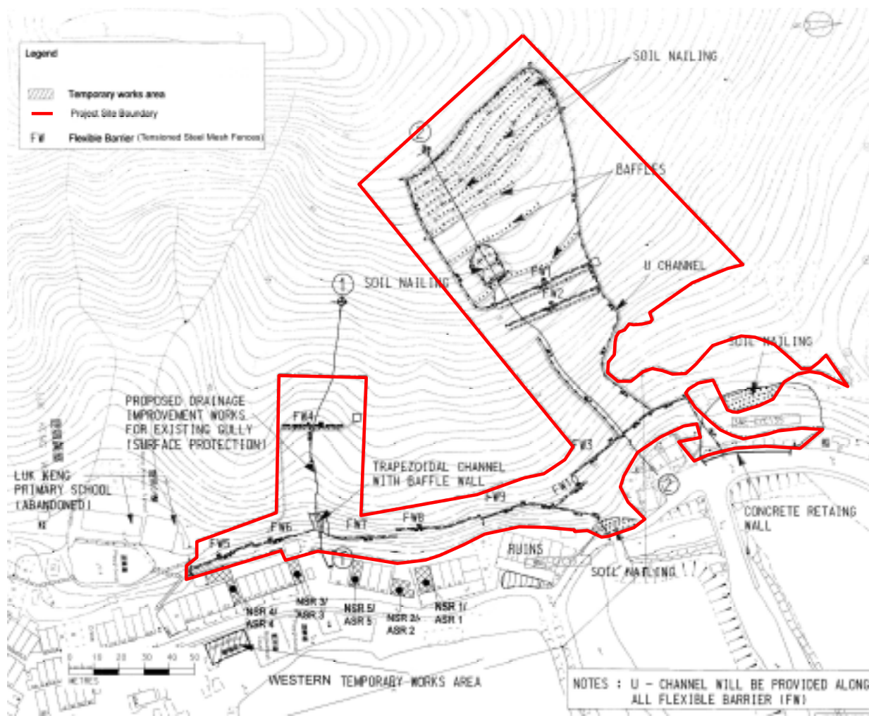
Figure 1 : Natural Terrain Hazard Mitigation Works in Luk Keng Wong UK – Project Layout
