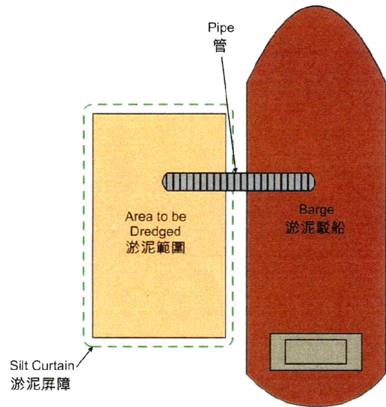
(a) Cage Type Silt Curtain Arrangement for Suction Dredging 吸管挖泥的淤泥屏障布置
