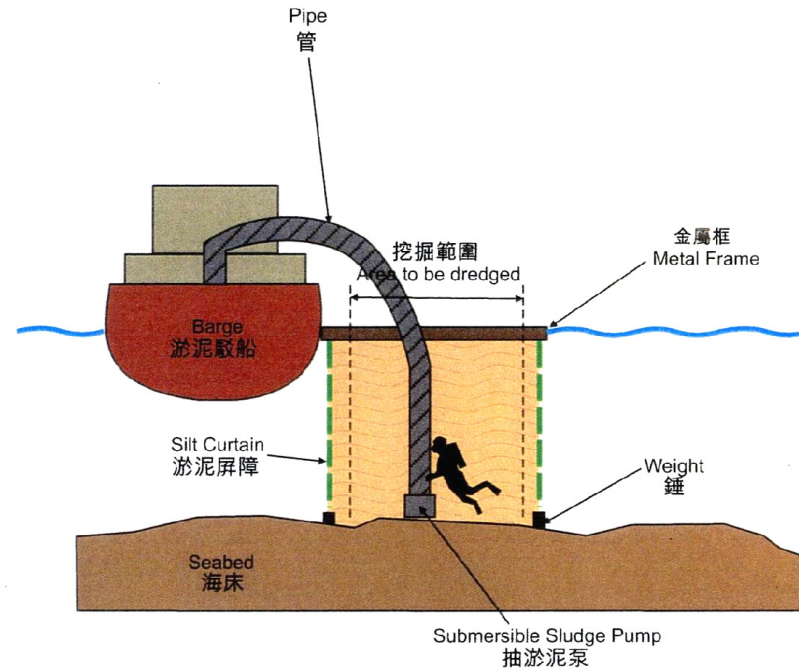
(b) Cross-section of Cage Type Silt Curtain Arrangement 淤泥屏障布置的橫切面
