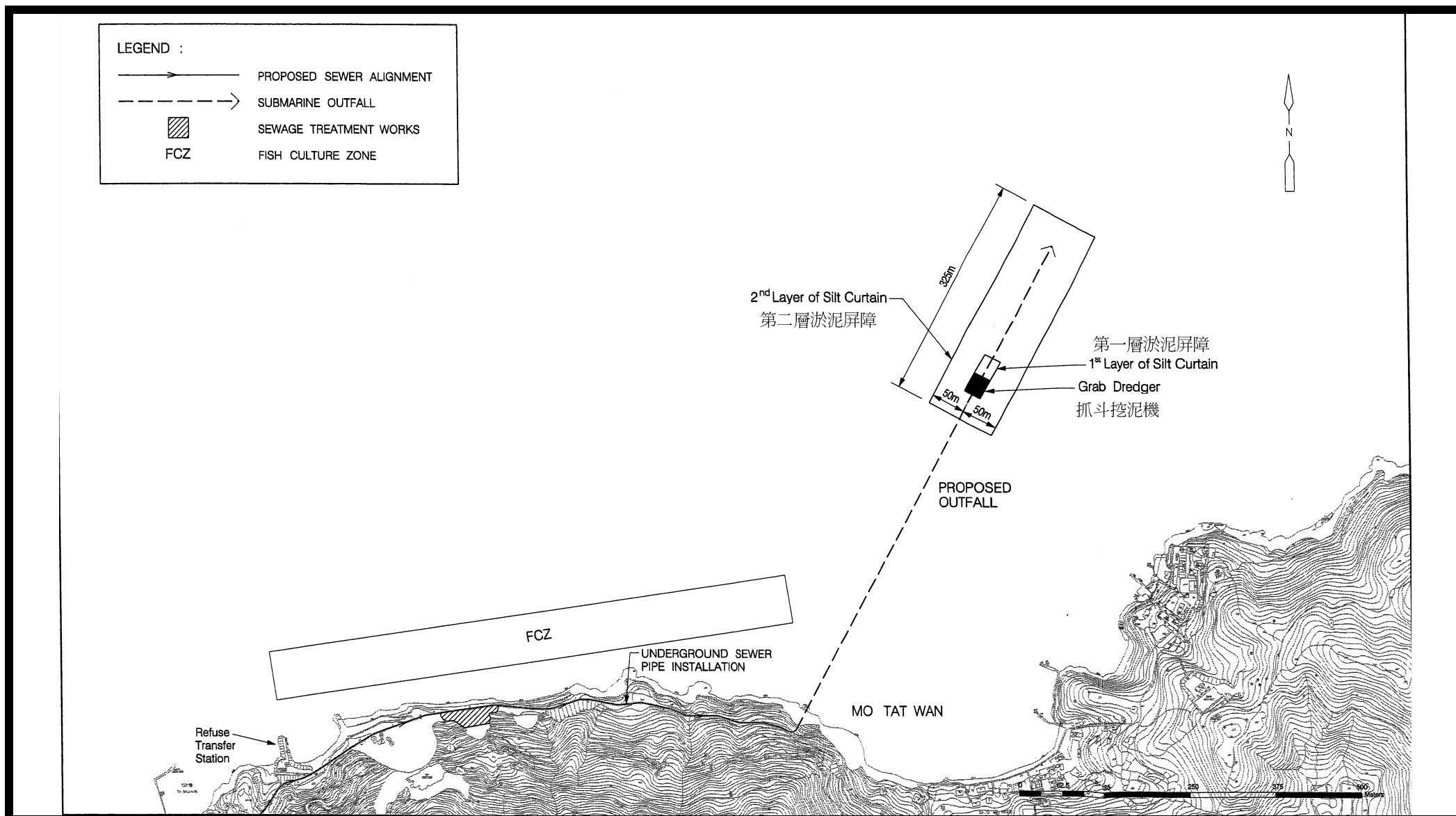
Figure 3: Arrangement of Silt Curtain during Construction
