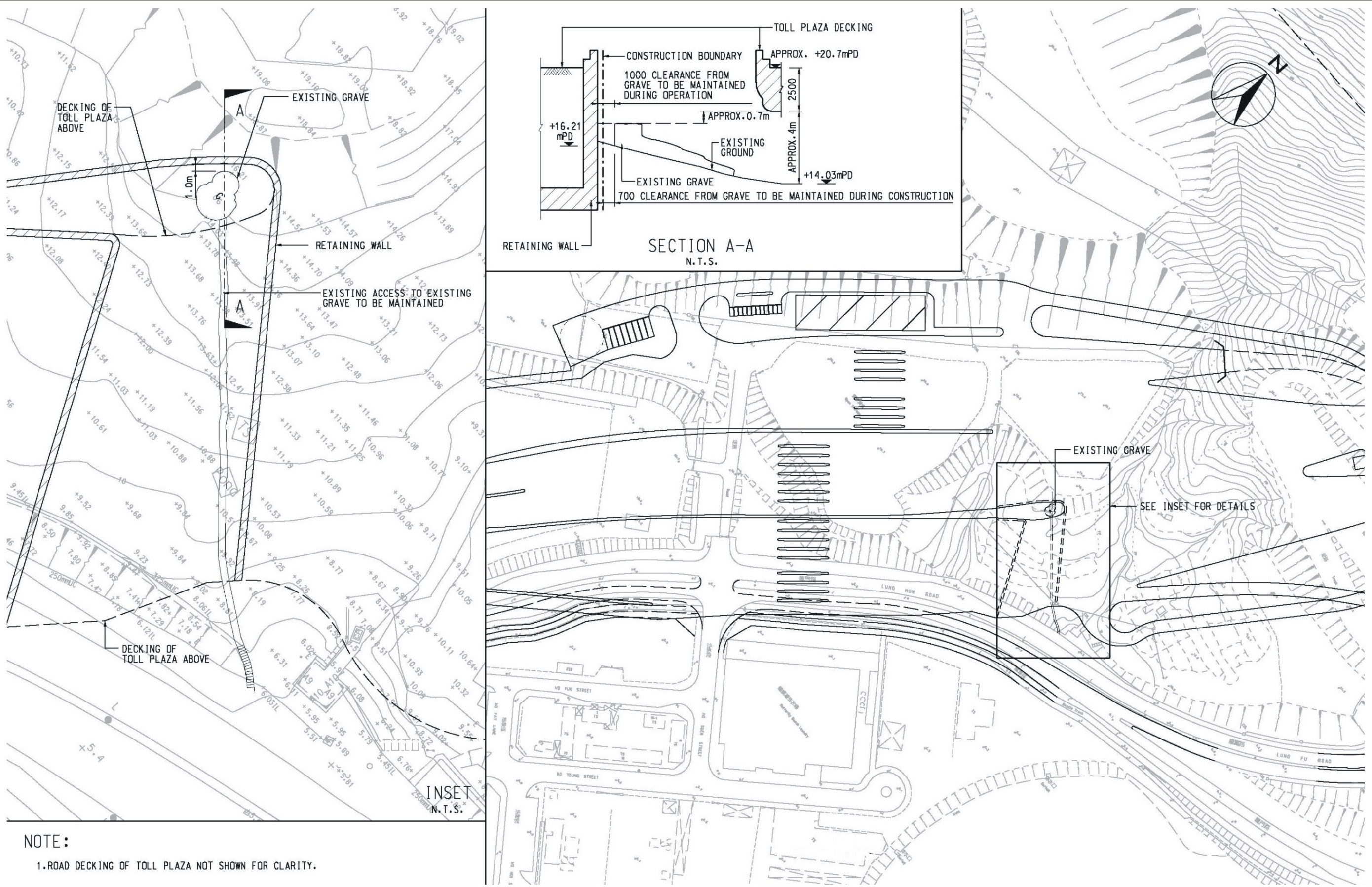
Figure 2 - Retaining walls arrangement at existing grave
