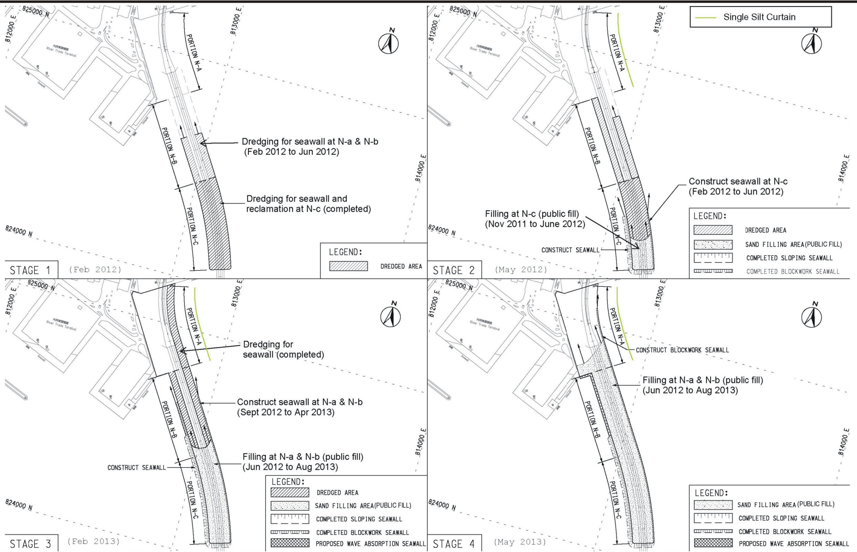
Figure 3 - Construction Sequence of Northern Landfall
