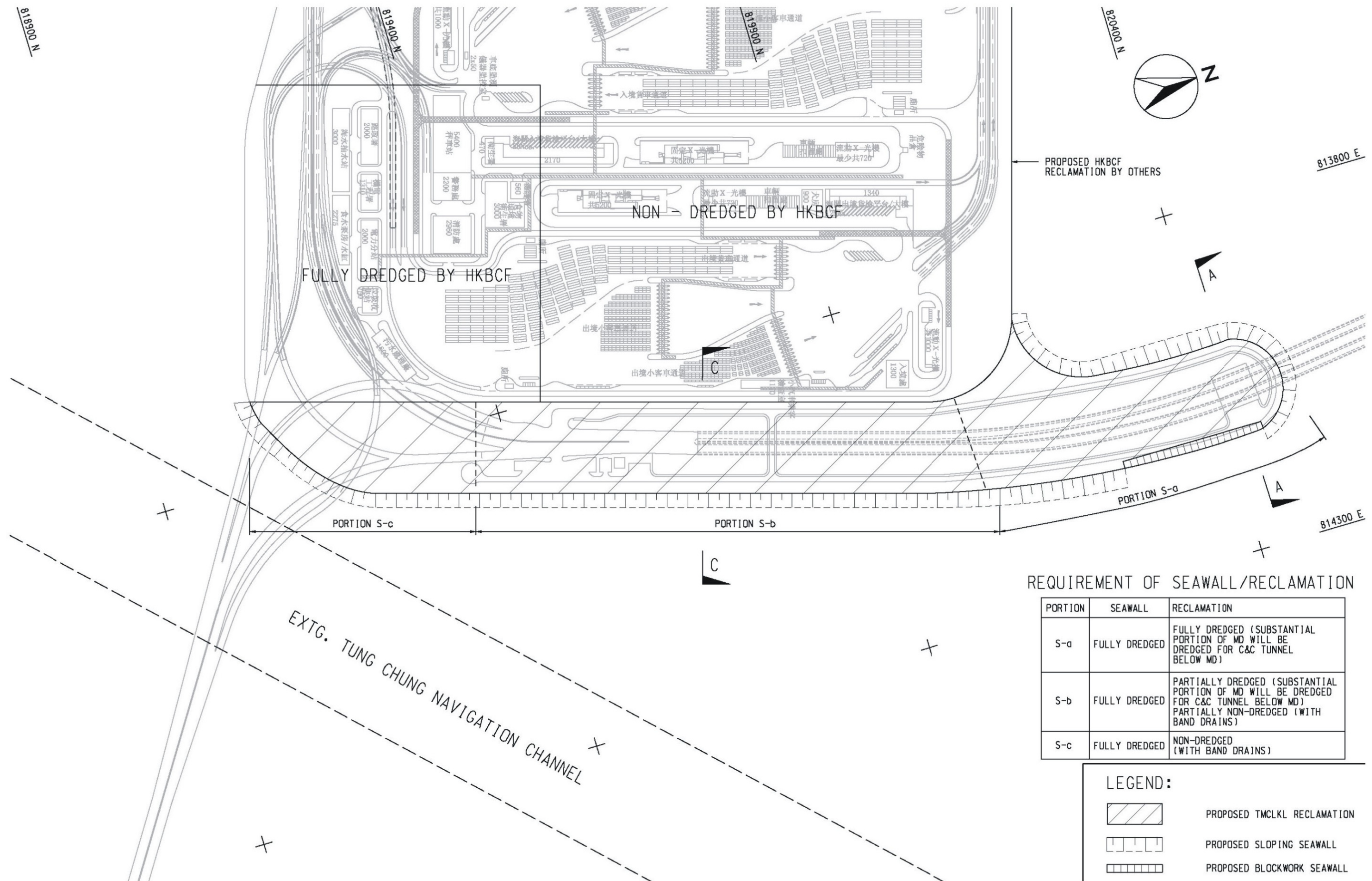
Figure 4 - General Layout of Southern Landfall
