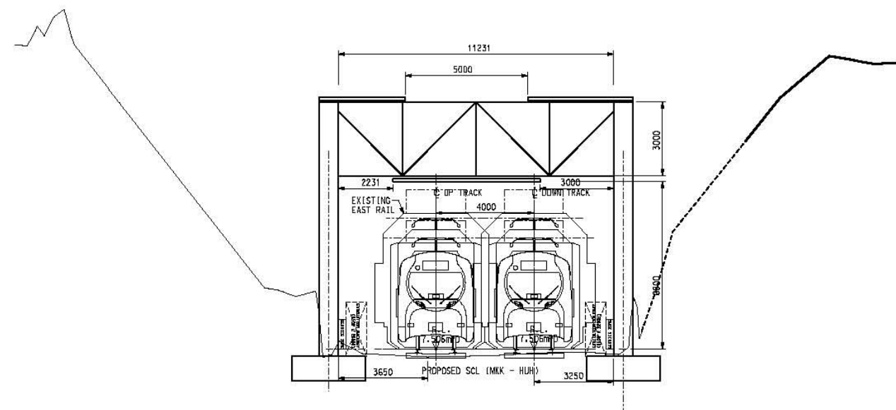
TYPICAL CROSS SECTION A
