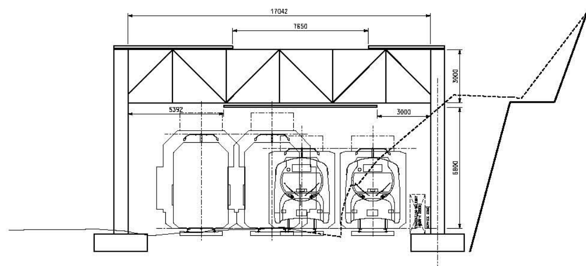
TYPICAL CROSS SECTION B
