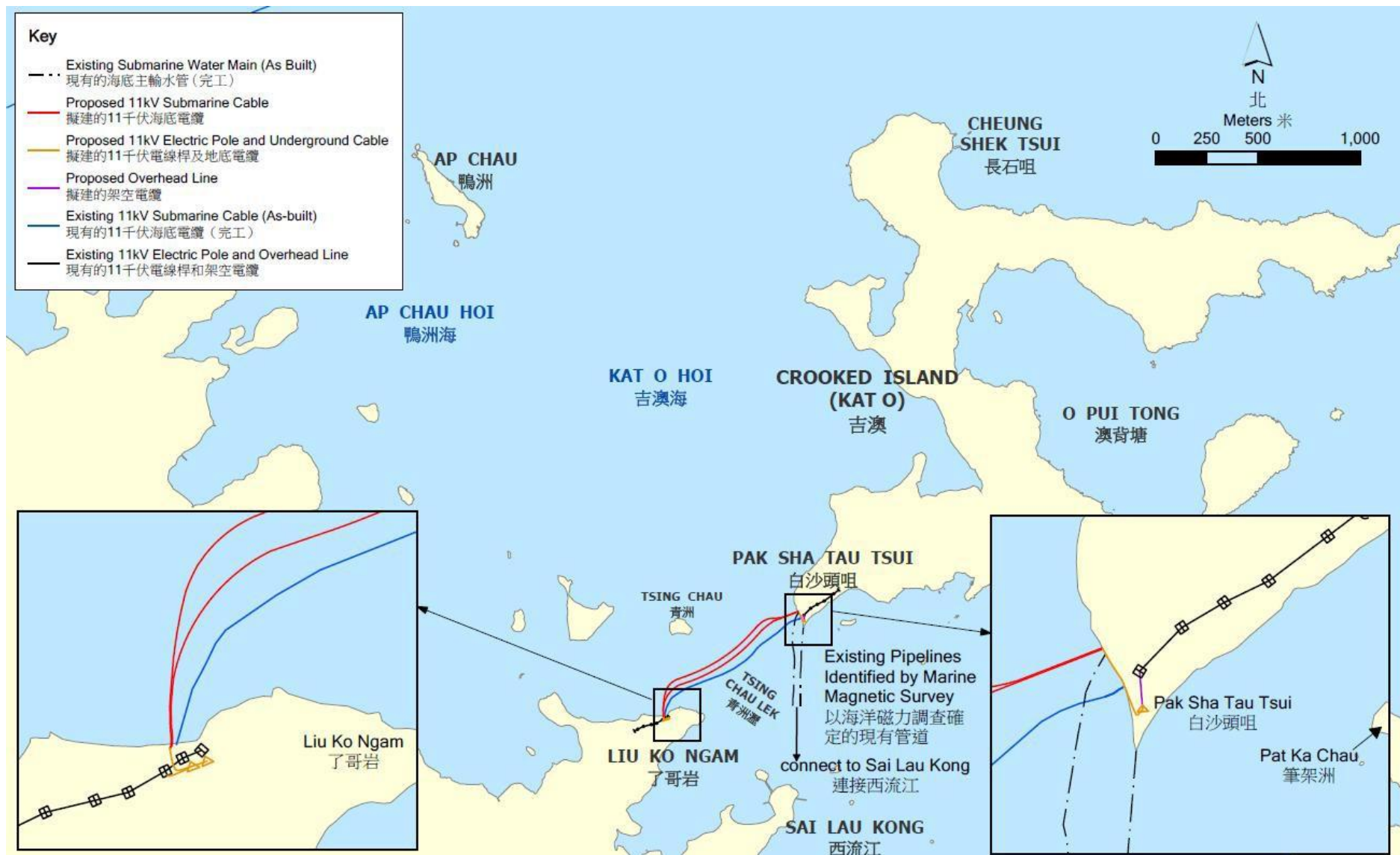
Figure 1 : Replacement of the Existing 11kV Submarine Cable Circuit Connecting Liu Ko Ngam and Pak Sha Tau Tsui at Kat O
