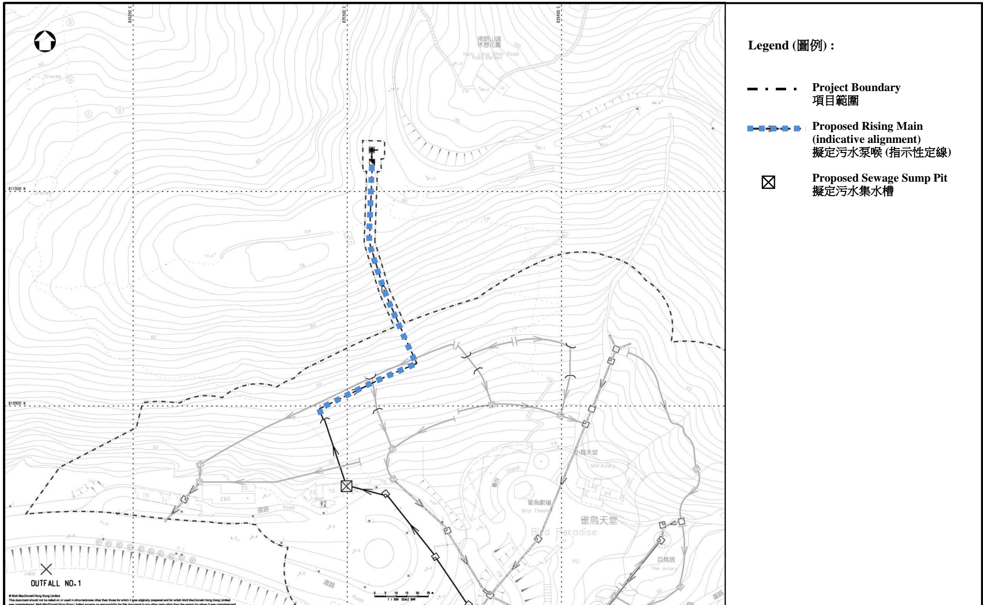
Figure 4: Location of Proposed Rising Main and Sewage Facilities 圖 4: 擬定污水泵喉及污水設施的位置
