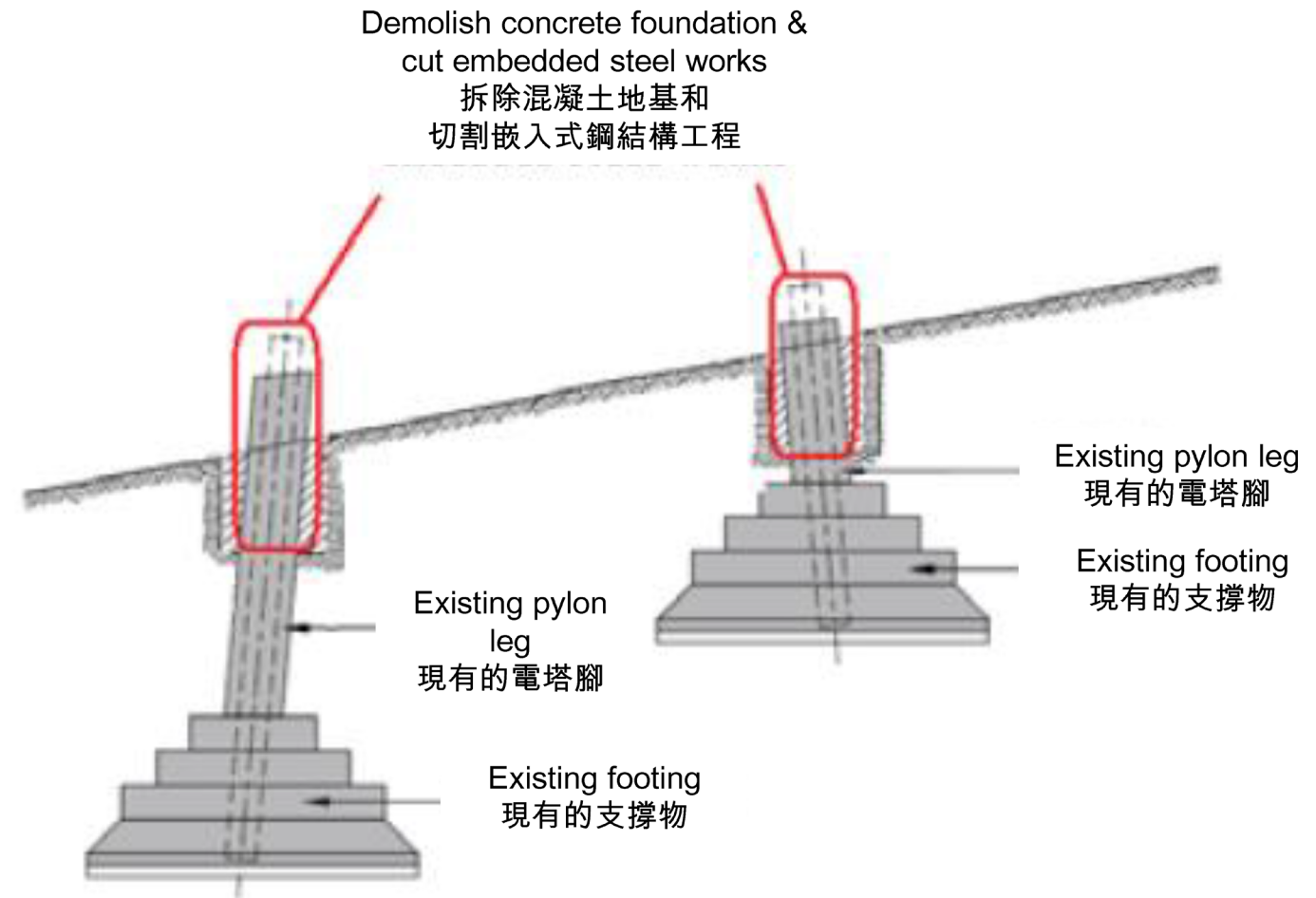
Removal of pylon foundations 拆除電塔地基
