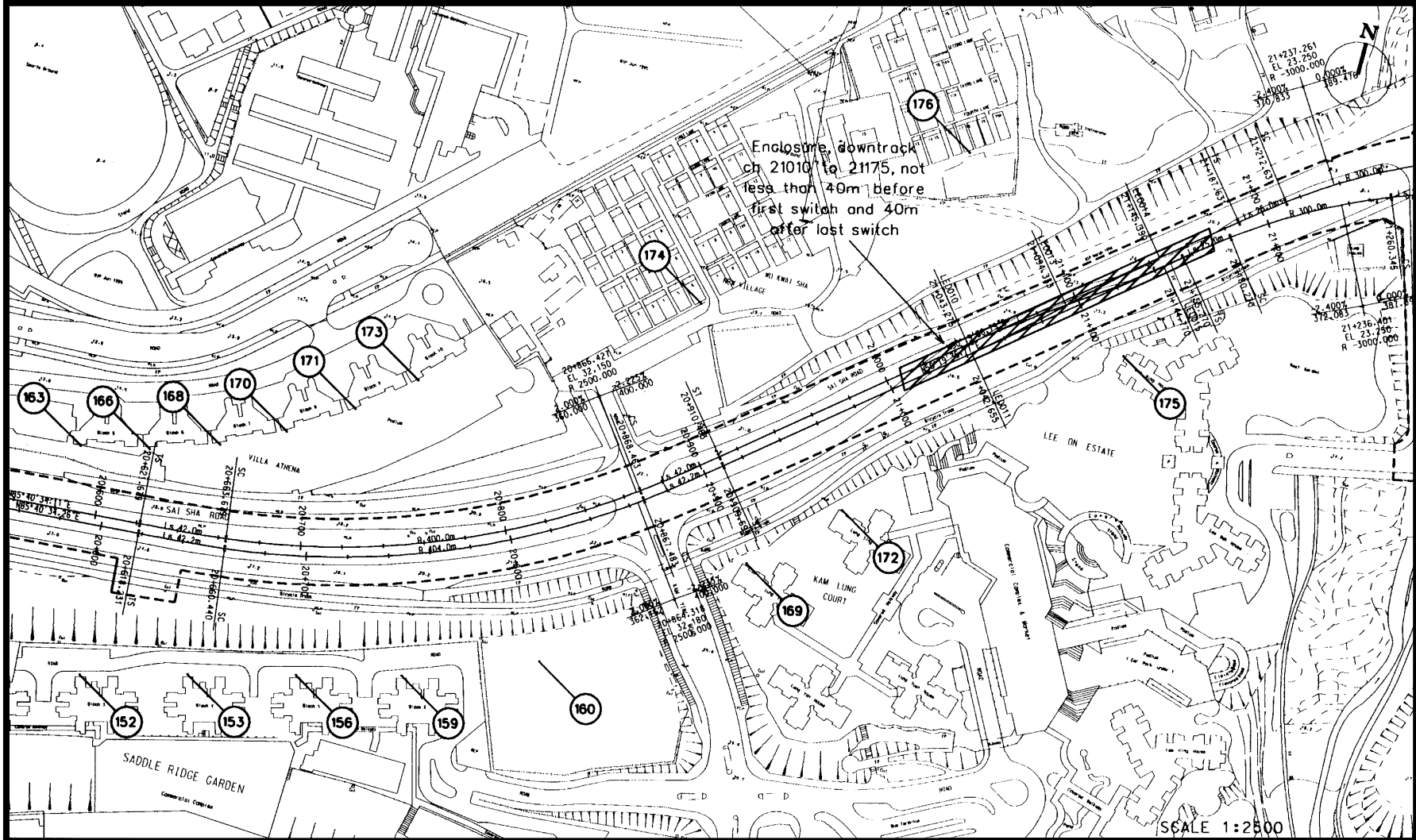
Figure 8 Noise Barriers and Enclosures (Extracted from Technical Annex F1 of the EIA Report)
