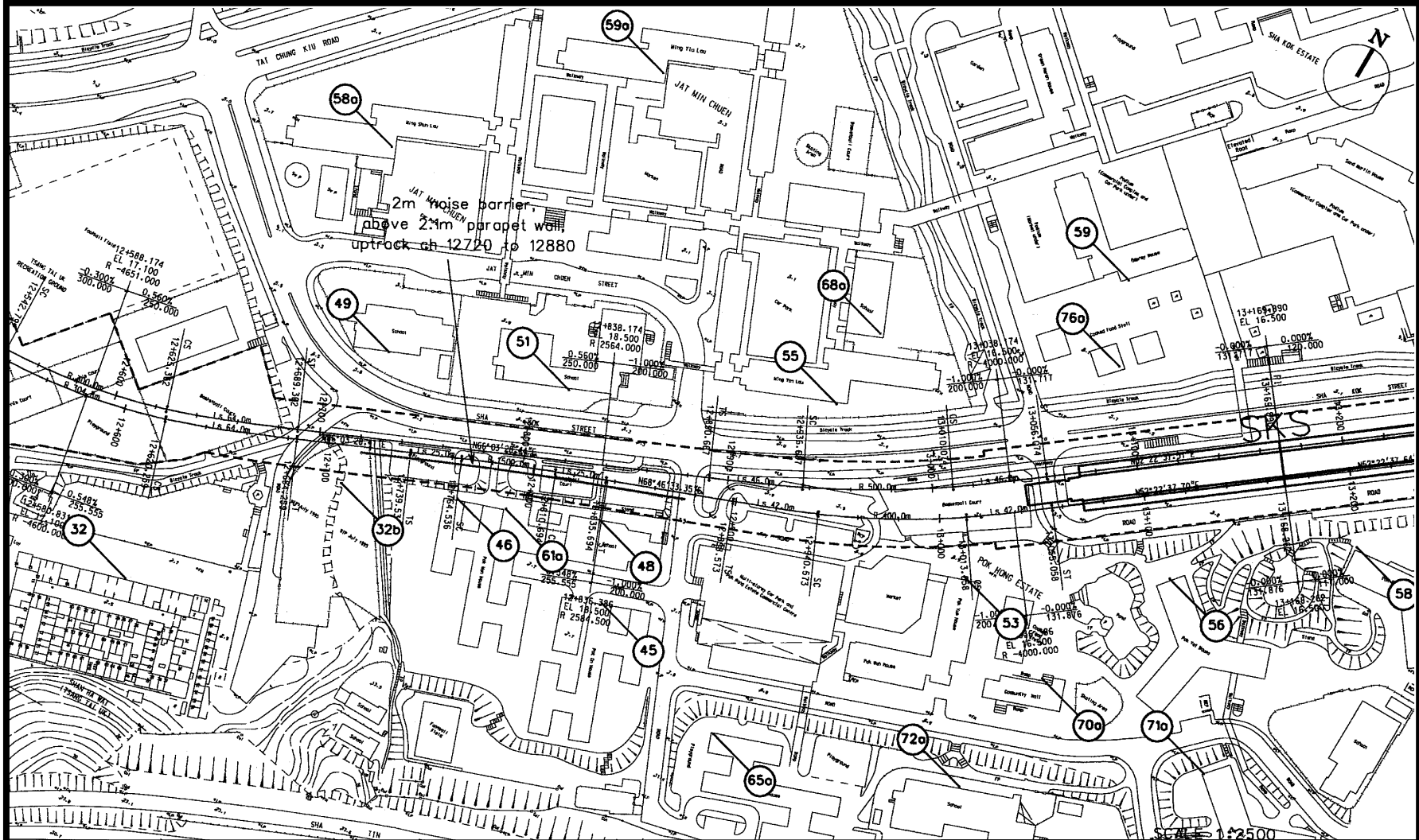
Figure 1 Noise Barriers and Enclosures (Extracted from Technical Annex F1 of the EIA Report)
