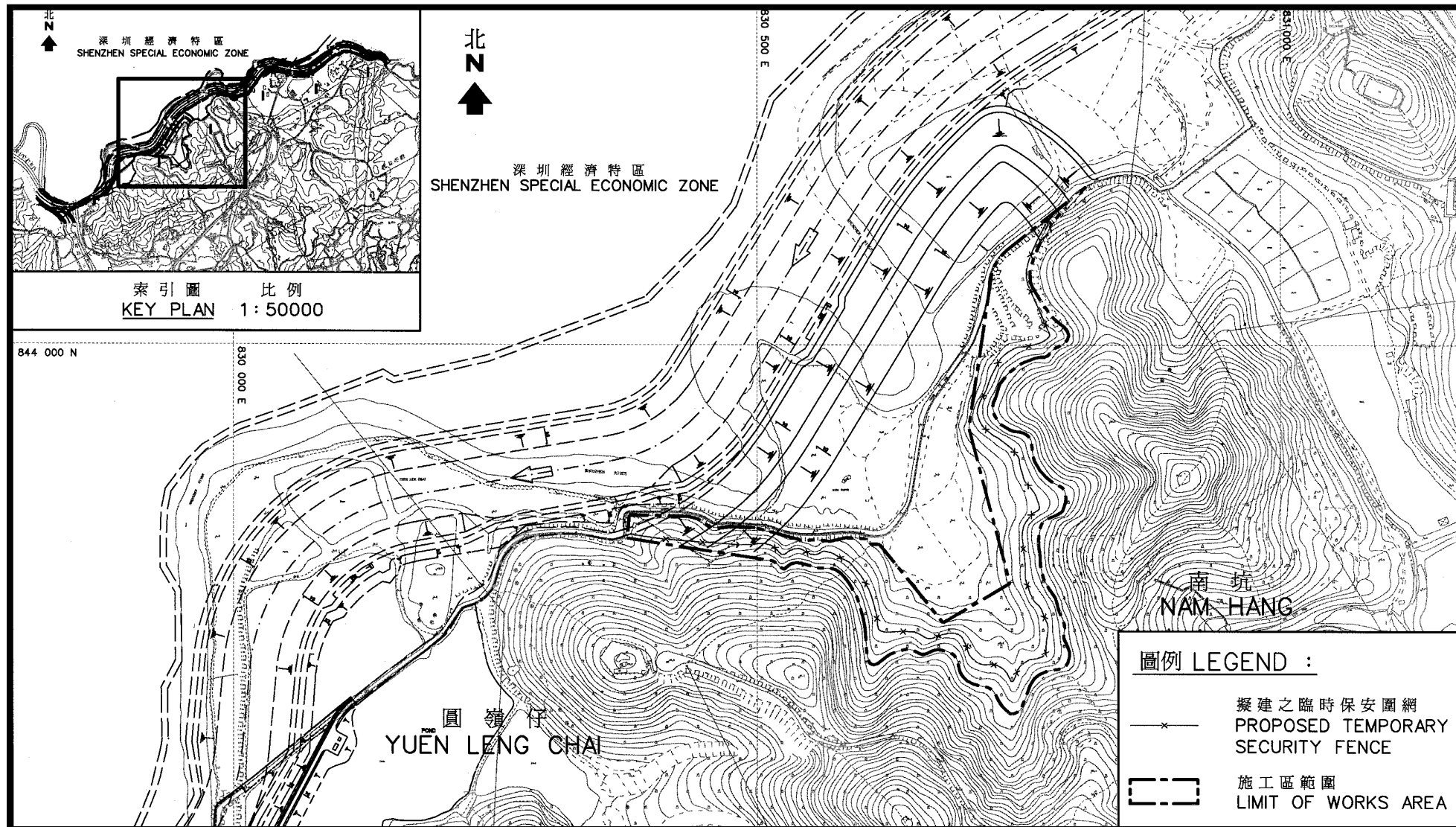
圖 1 治理深圳河第三期工程 - 南坑臨時保安圍網 Figure 1 Shenzhen River Regulation Project Stage III - Temporary Security Fence at Nam Hang
