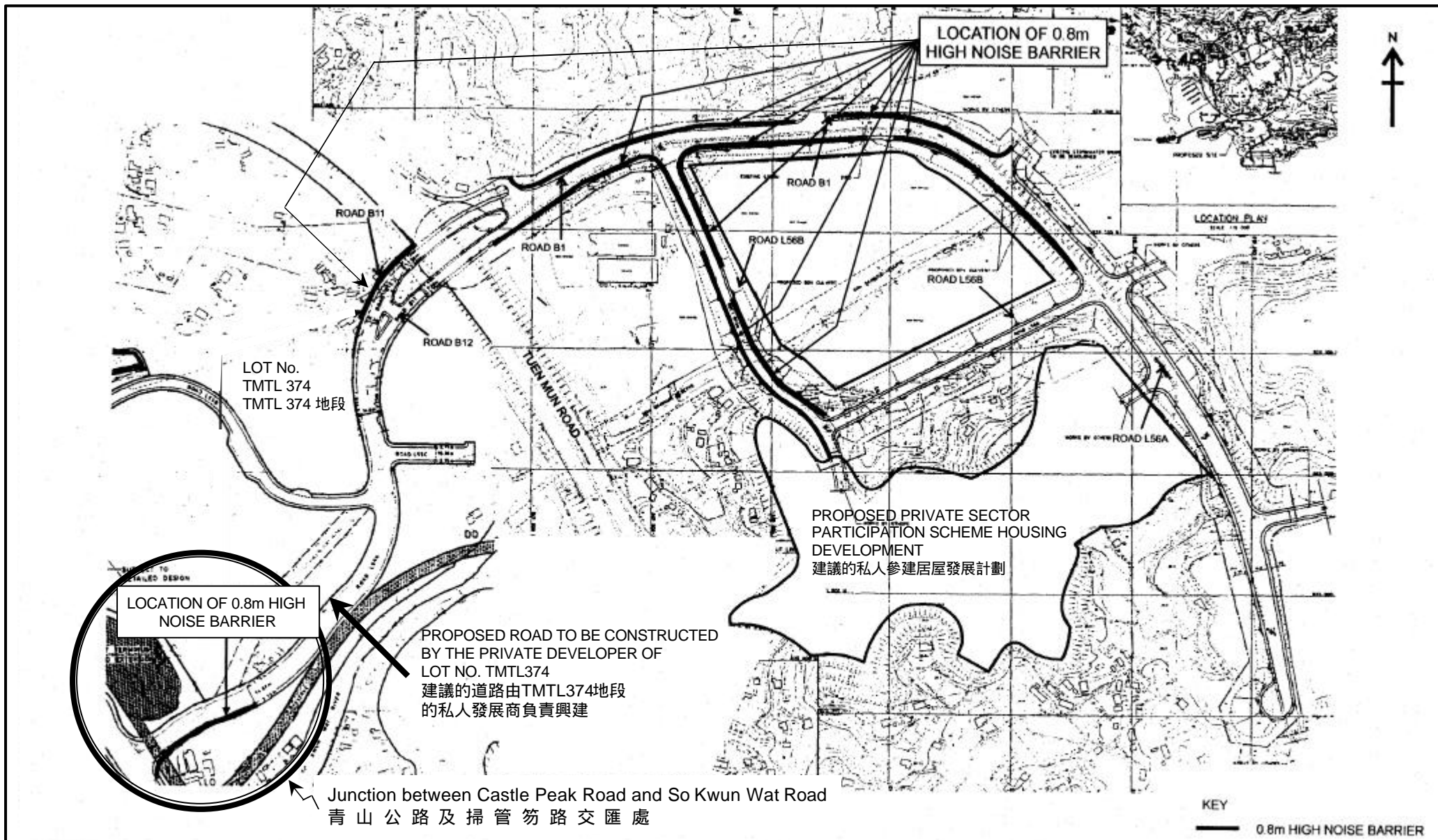
Construction of Roads and Drains to Serve the Housing Development in Area 56, Tuen Mun Improvement Works at Junction between Castle Peak Road and So Kwun Wat Road Plan showing location of noise barrier
